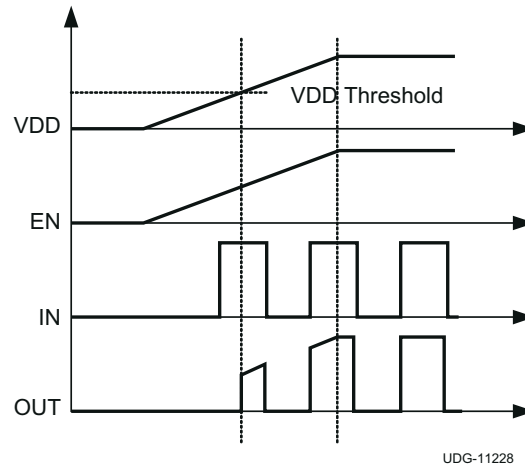
Figure 7-2. Power-Up Sequence
