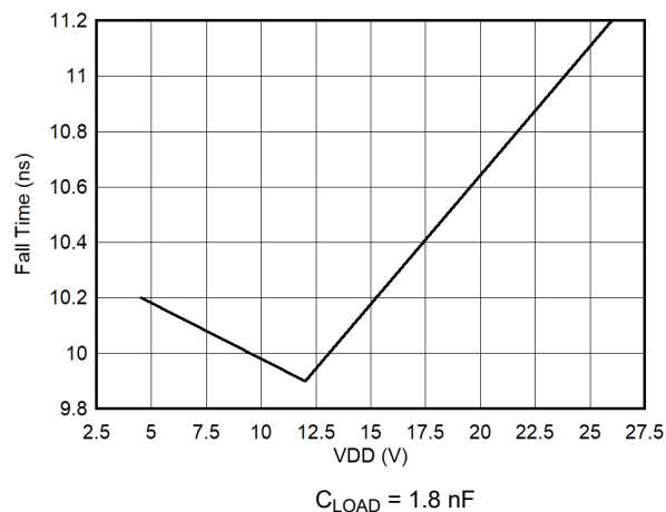
Figure 5-15. Output Fall Time vs VDD
