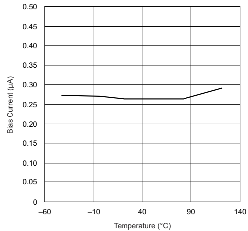
Figure 5-4. I VSENSE Bias Current vs Junction Temperature
