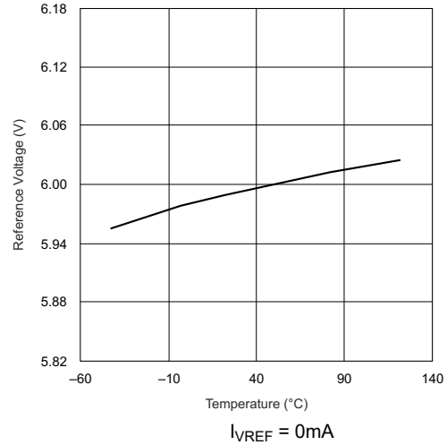
Figure 5-2. V VREF vs Junction Temperature
