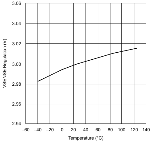
Figure 5-3. V VSENSE Regulation vs Junction Temperature
