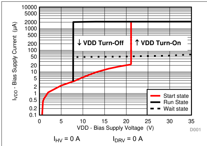
Figure 5-1. Bias Supply Current vs. Bias Supply Voltage
