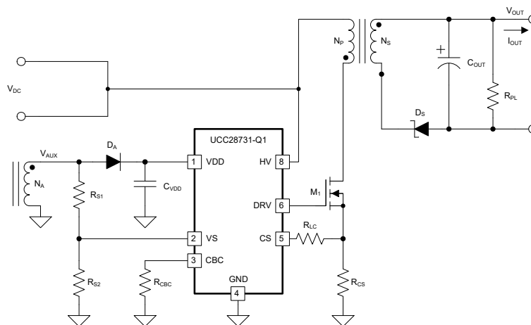
Figure 3-1. Simplified Schematic
