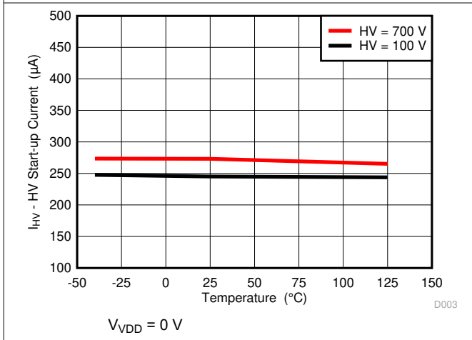
Figure 5-3. HV Start-up Current vs. Temperature
