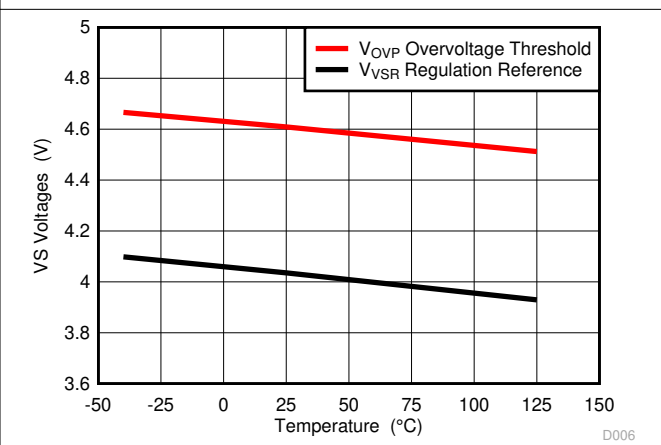
Figure 5-6. VS Voltages vs. Temperature
