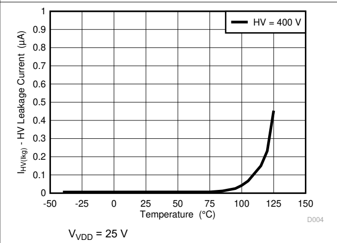
Figure 5-4. HV Leakage Current vs. Temperature
