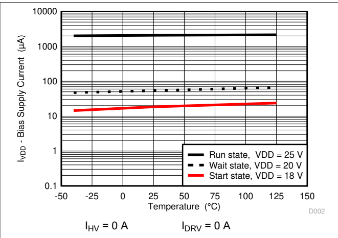
Figure 5-2. Bias Supply Current vs. Temperature
