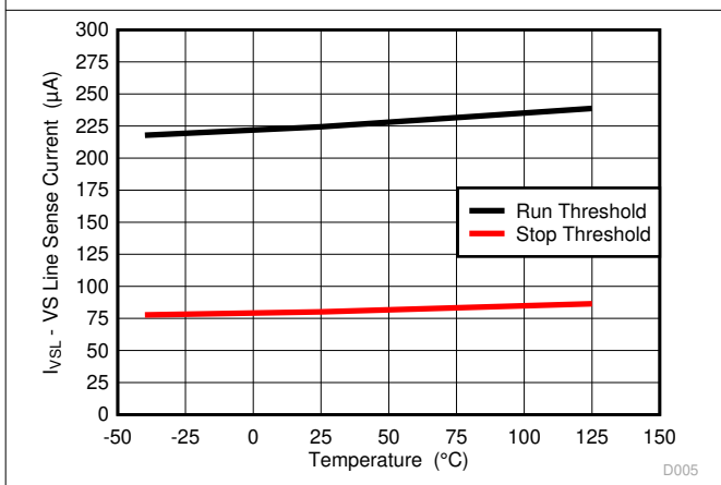
Figure 5-5. VS Line-Sense Current vs. Temperature
