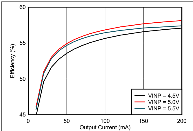
Figure 6-7. Efficiency vs Load Current ( I_{VCC} ): V_{CC} = 5.5V , T_A = 25^\circ C , C_{OUT2} = 22\mu F
