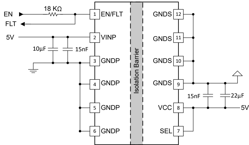
Figure 8-1. Typical Application
