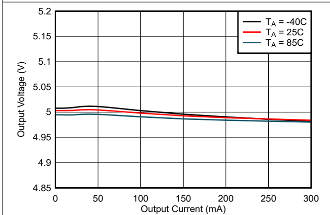
Figure 6-11. Output Voltage Regulation ( V_{VCC} ) vs Load Current ( I_{VCC} ): V_{CC} = 5.0V , V_{INP} = 5.0V , C_{OUT2} = 22\mu F
