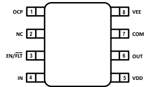
Figure 4-1. UCC5713xB 8-Pin SOIC D Package Top View
