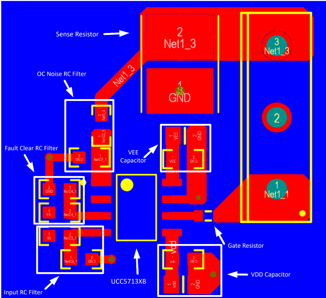
Figure 7-5. Layout Example: UCC5713x
