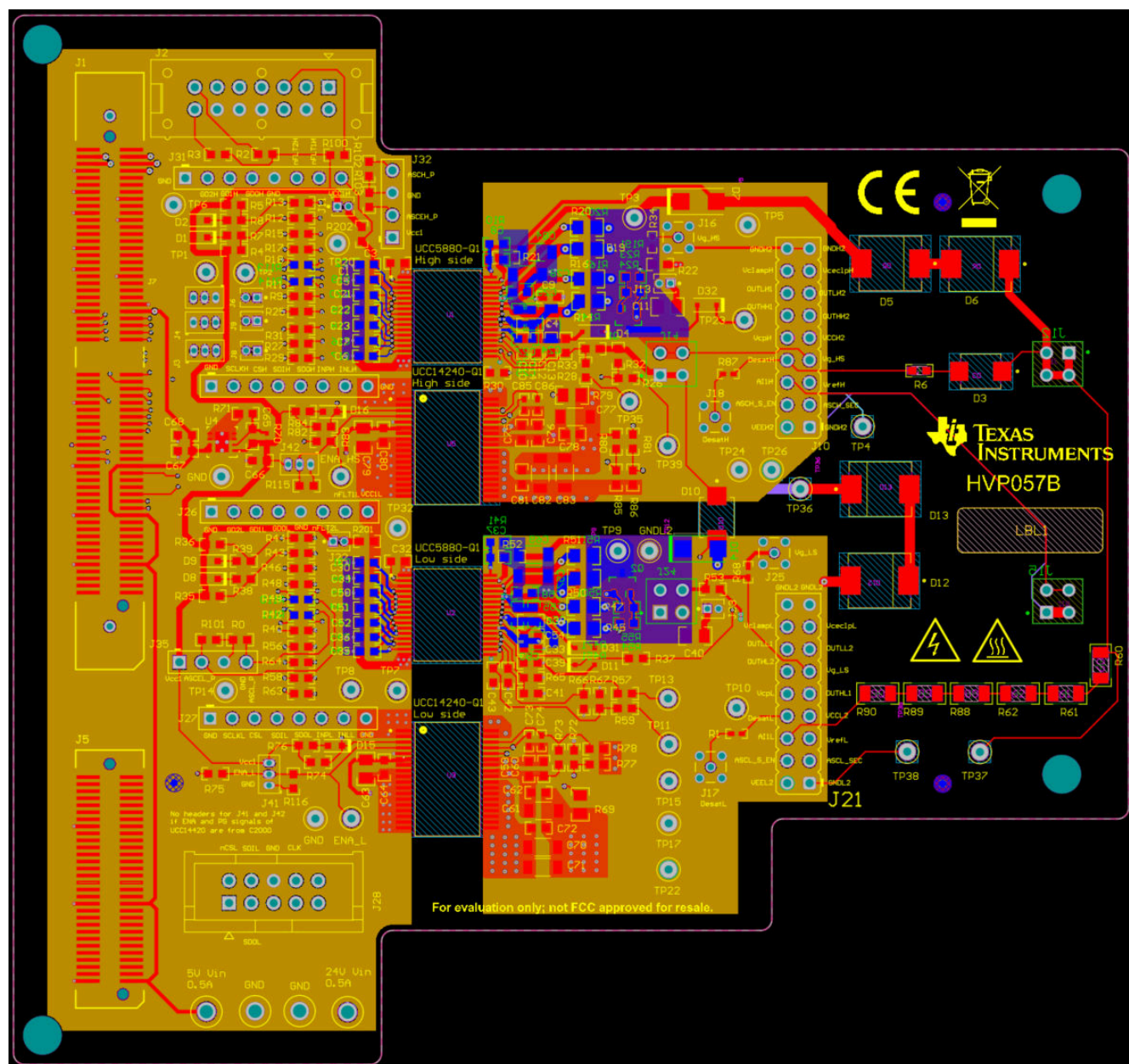
Figure 6-1. 2D Layout Example
