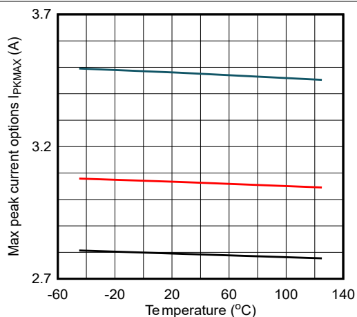
Figure 6-7. Maximum Primary Peak Current vs Junction Temperature
