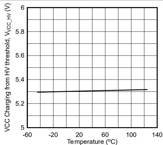
Figure 6-2. VCC Threshold for Charging From HV Pin vs Junction Temperature
