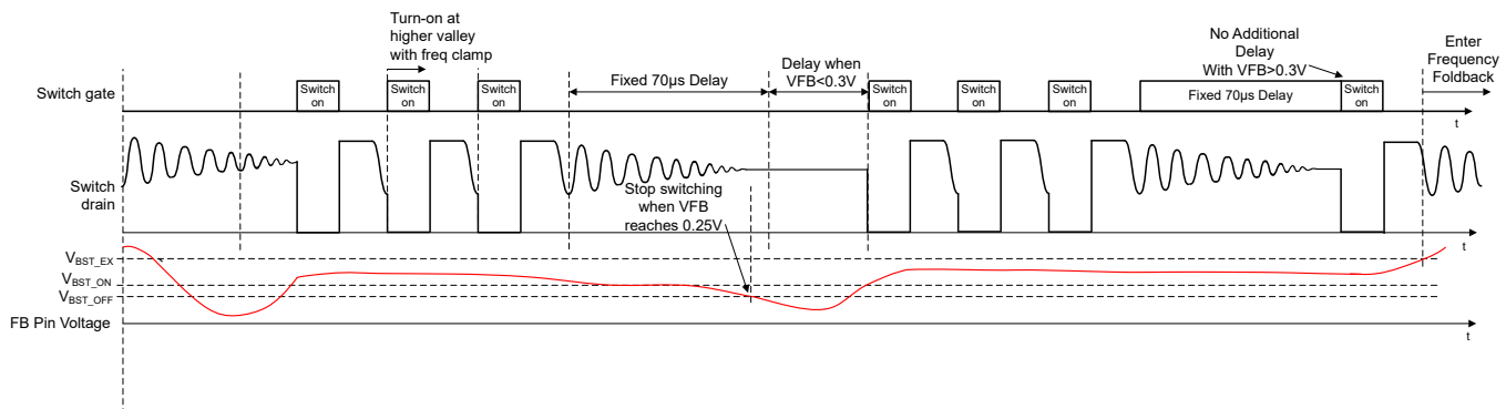
Figure 7-6. Burst Mode Entry and Exit Waveforms
