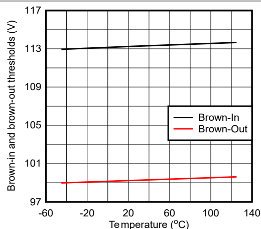
Figure 6-8. Brownin and Brownout Thresholds vs Junction Temperature
