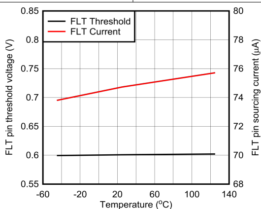
Figure 6-9. FLT Pin Voltage and Current vs Junction Temperature
