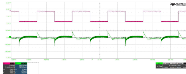
Figure 8-9. Load Transient at 230VAC and 20V Output
