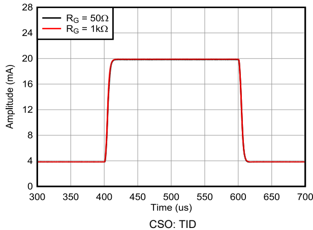
Figure 5-3. Step Response
