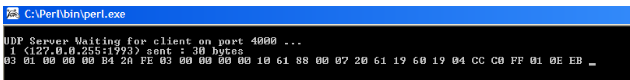
Figure 6: Sample packet as shown by udp_receive.pl
