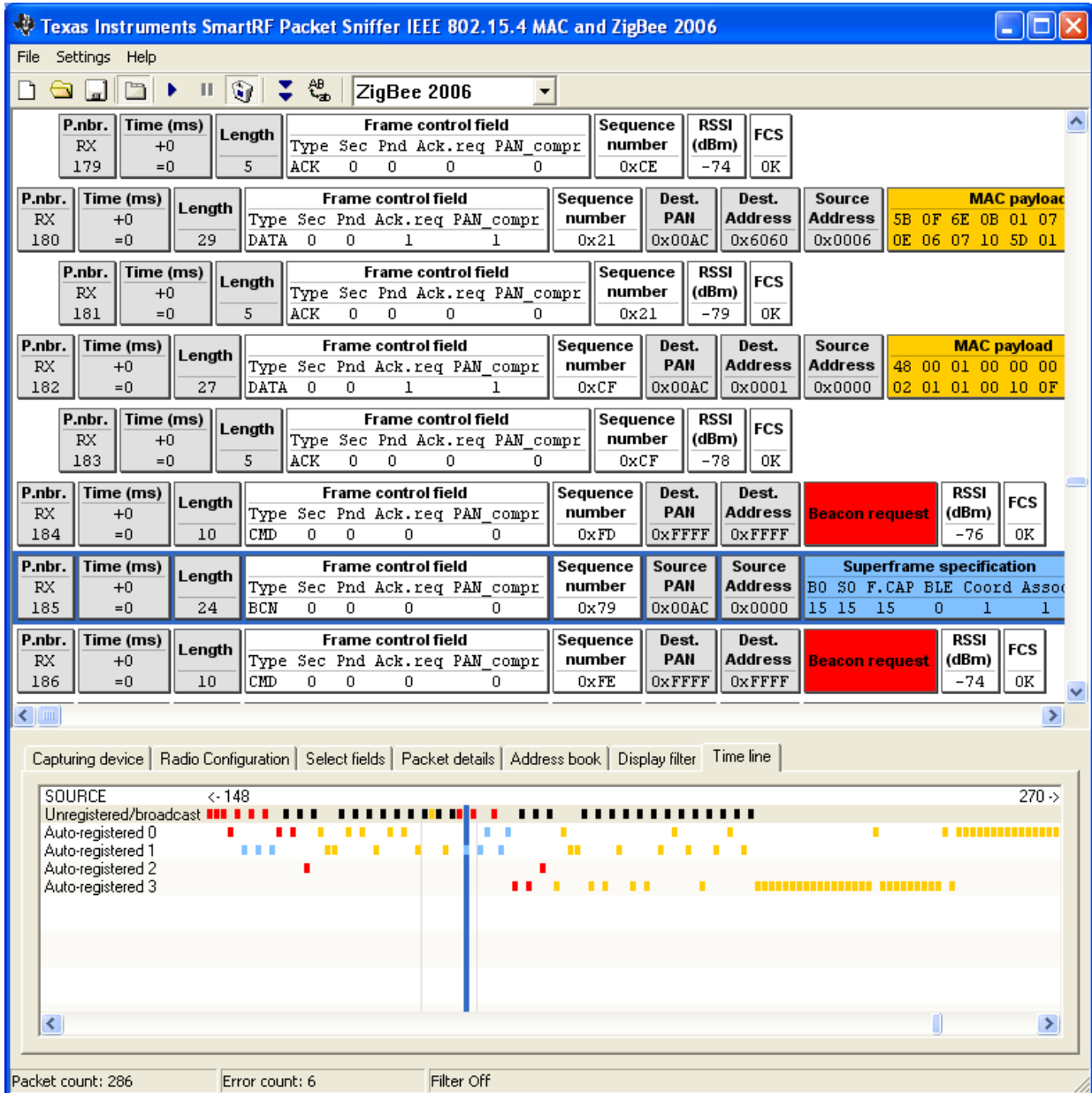
Figure 3: Packet sniffer screenshot from the IEEE802.15.4/ZigBee protocols
