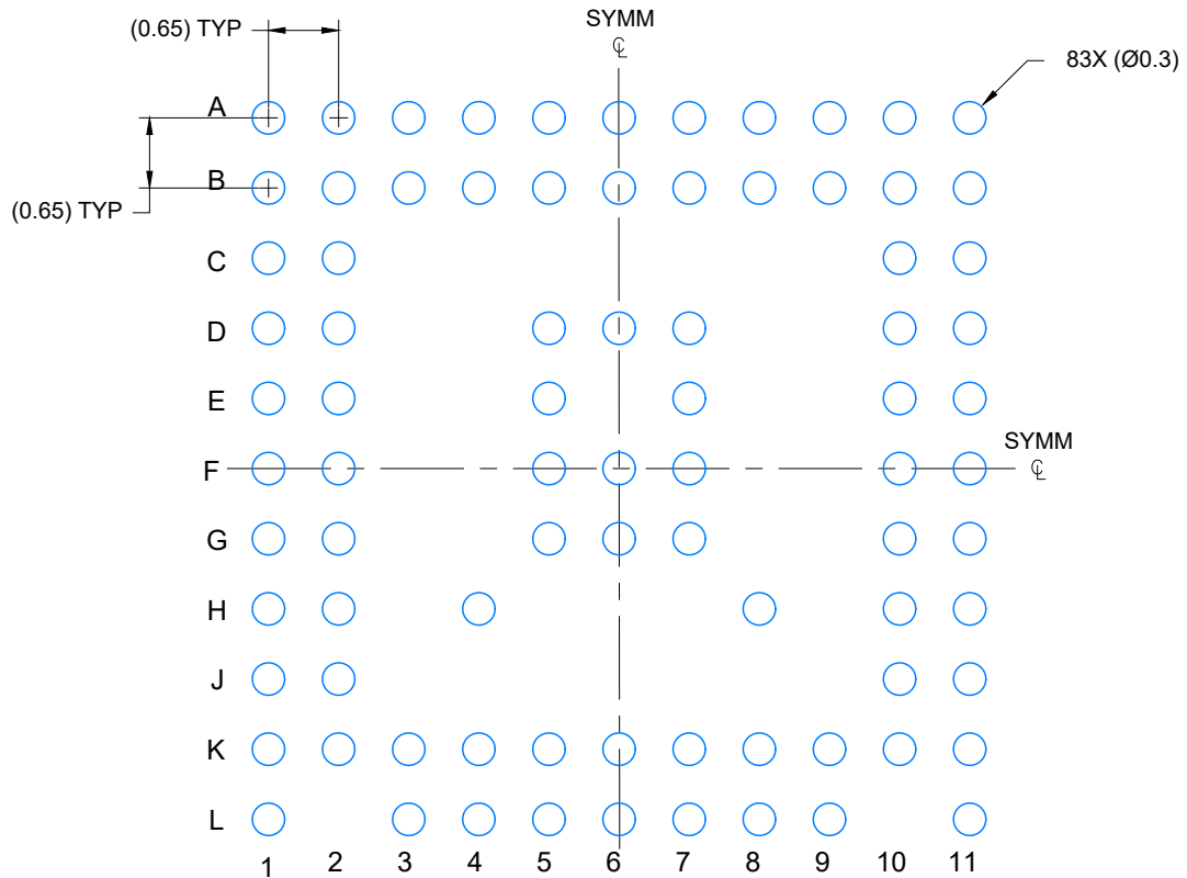
LAND PATTERN EXAMPLE SCALE: 13X
