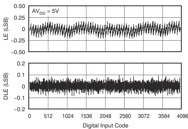
Figure 7-4. DAC7311 12-Bit Linearity Error and Differential Linearity Error vs Code ( 25^\circ\text{C} )
