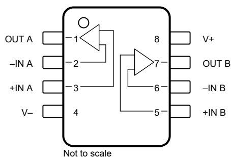
Figure 4-1. Pin Diagram
