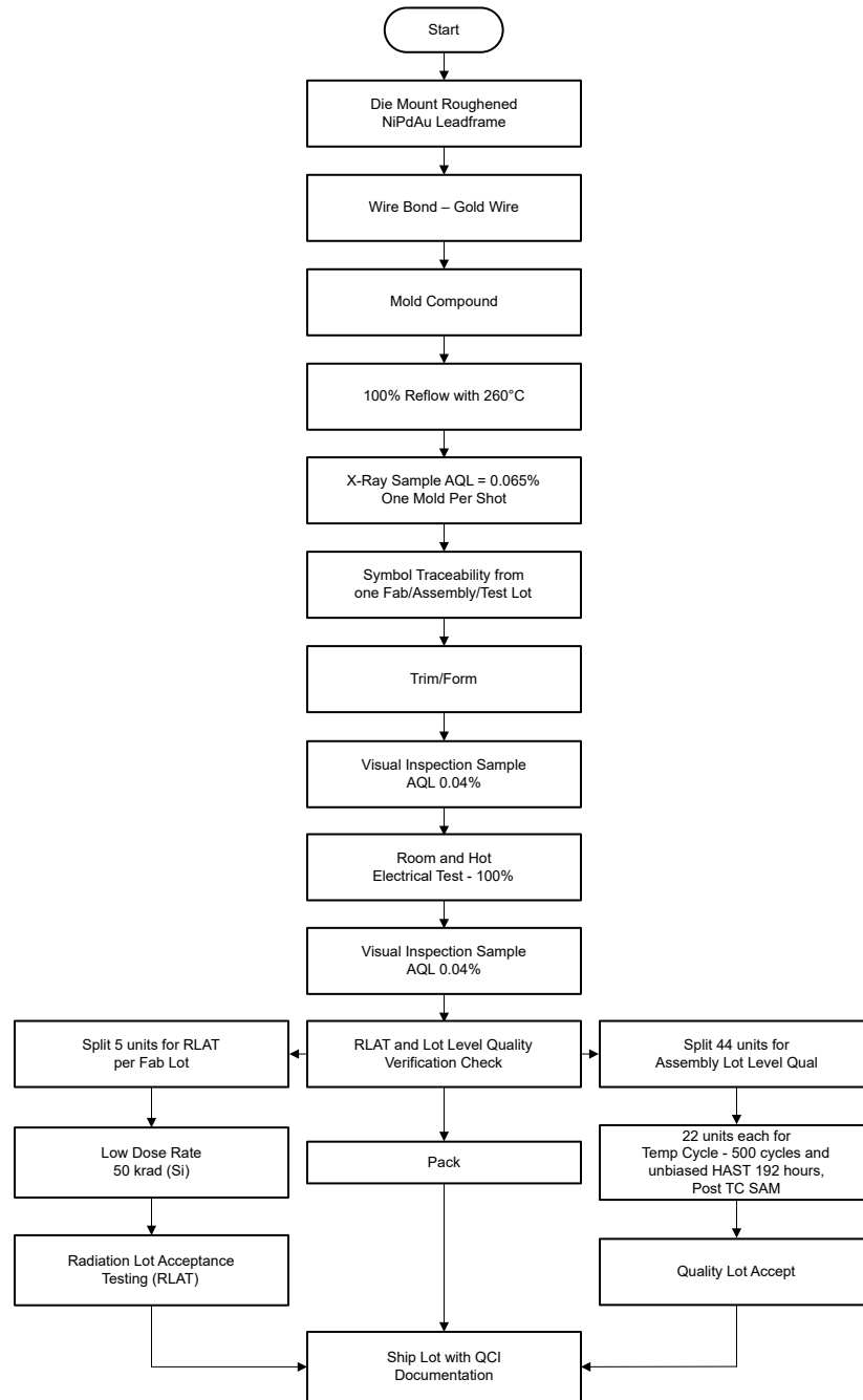
Figure 2-1. TMP9R01-SEP Space Enhanced Plastic Production Flow Chart
