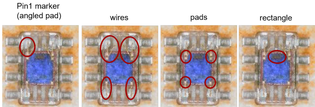
Figure 11-4. Identifying DTS Package Orientation - Backside
