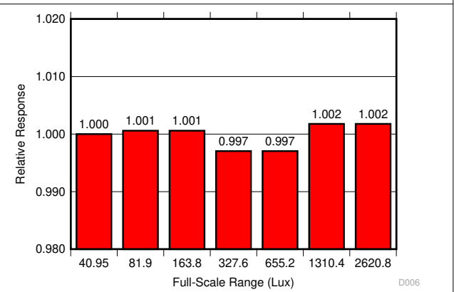
Figure 5-7. Full-Scale-Range Matching: Lowest 7 Ranges
