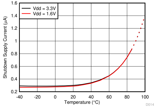
Figure 5-21. Shutdown Current vs Temperature (Grade 3)
