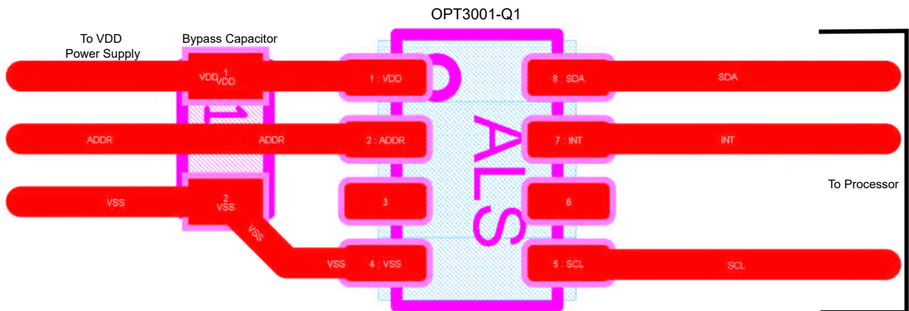
Figure 8-8. OPT3001-Q1 SOT-5X3 Layout Example
