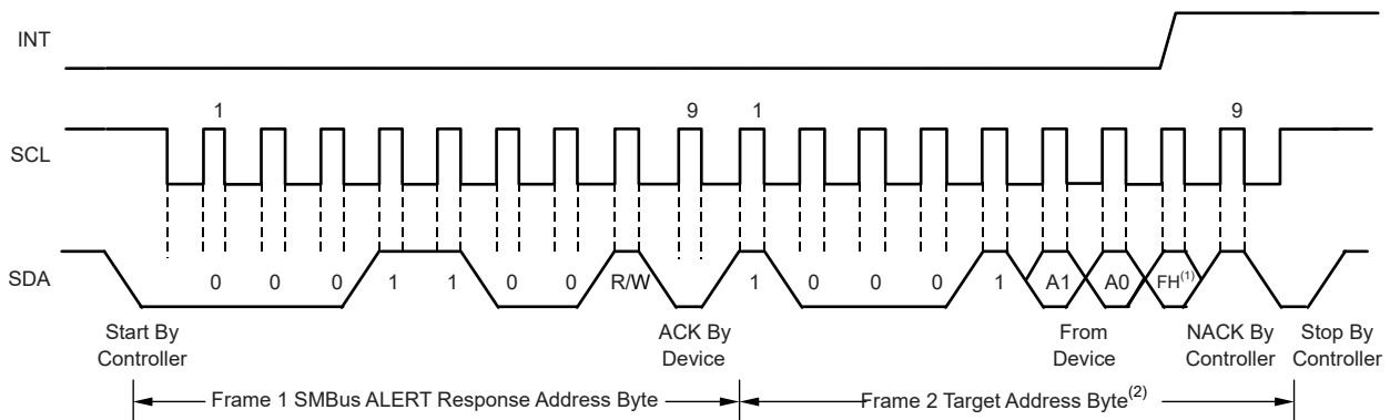
Figure 6-4. Timing Diagram for SMBus Alert Response
