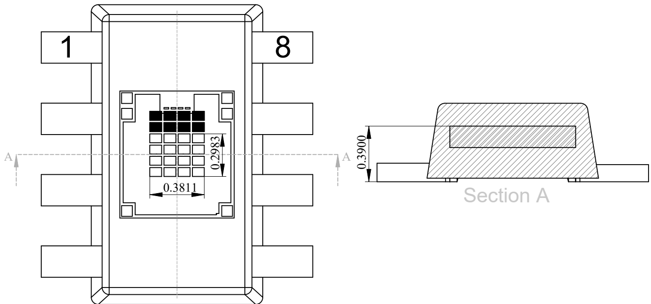
Figure 11-3. Package Orientation Visual Reference of Pin 1 (Top View) & Sectional View
