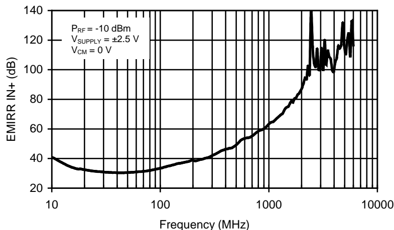
Figure 1. OPA627 EMIRR IN+ vs Frequency
