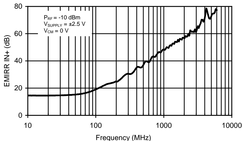
Figure 1. TLV2211 EMIRR IN+ vs Frequency
