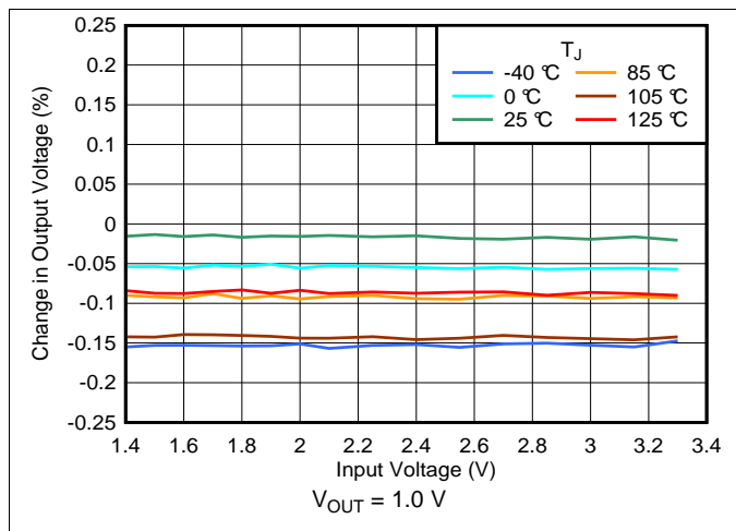
Figure 1. Output Accuracy Over Temperature, YKA Package
