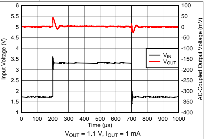
Figure 14. V_{IN} Transient
