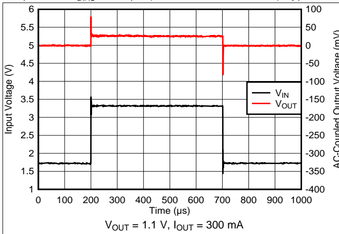
Figure 13. V_{IN} Transient
