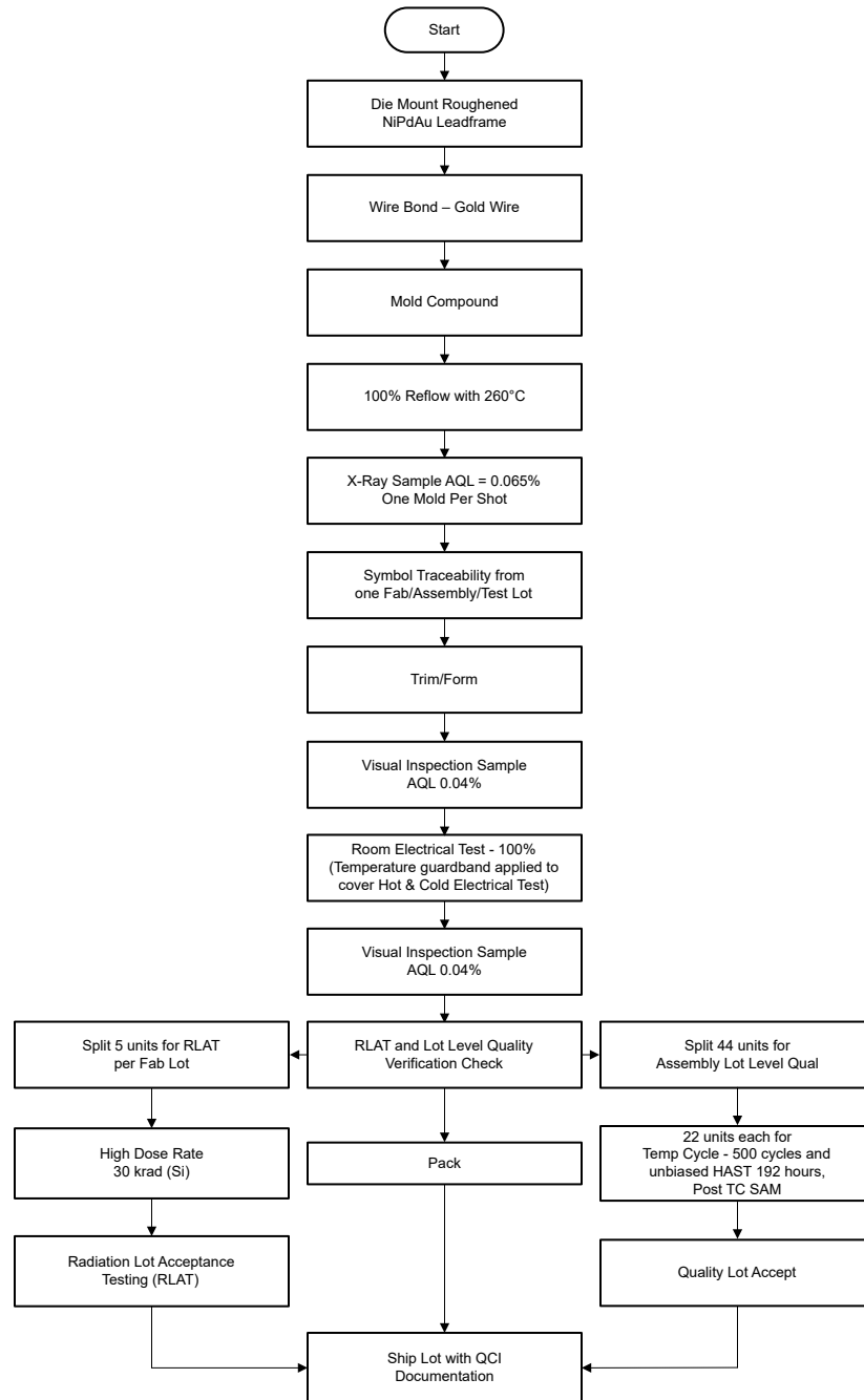
Figure 2-1. SN54SC8T164-SEP Space Enhanced Plastic Production Flow Chart
