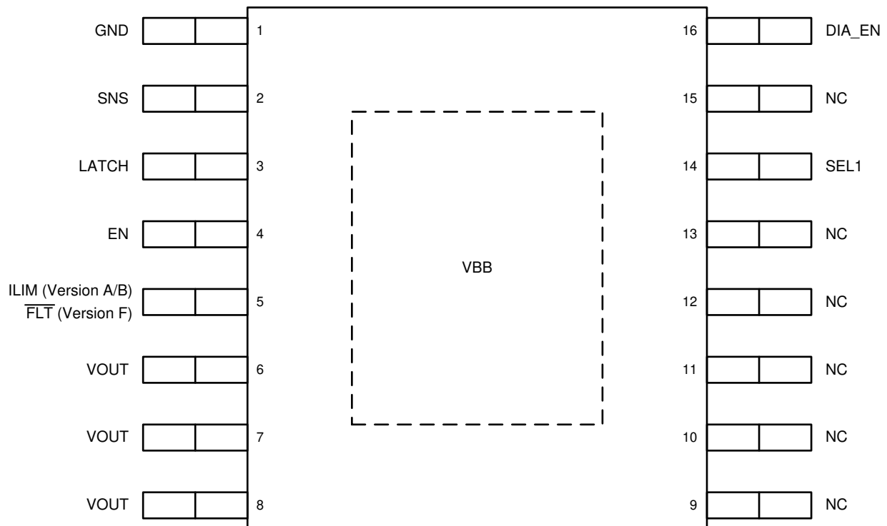
Figure 4-1. Pin Diagram
