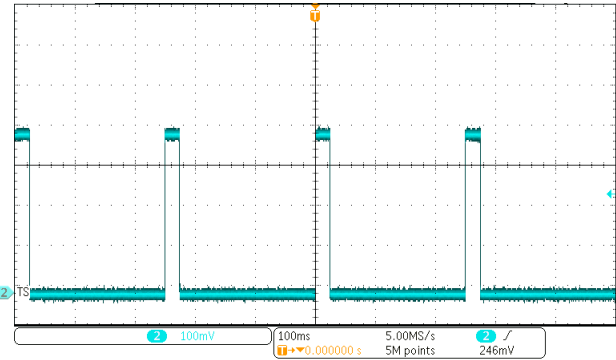
VIN = 5V Figure 10-21. TS Biasing and Voltage Behavior when VIN is Present
