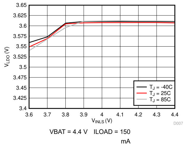
Figure 8-12. LDO Line Regulation (VLDO = 3.6 V)
