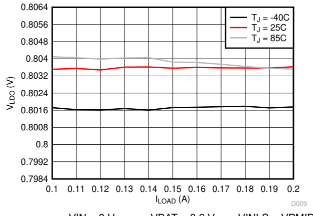
Figure 8-6. LDO Load Regulation (VLDO = 0.8 V)
