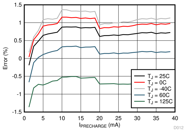
Figure 8-3. Pre-Charge Current Accuracy vs. IPRECHARGE Setting (ICHARGE_RANGE = 0)
