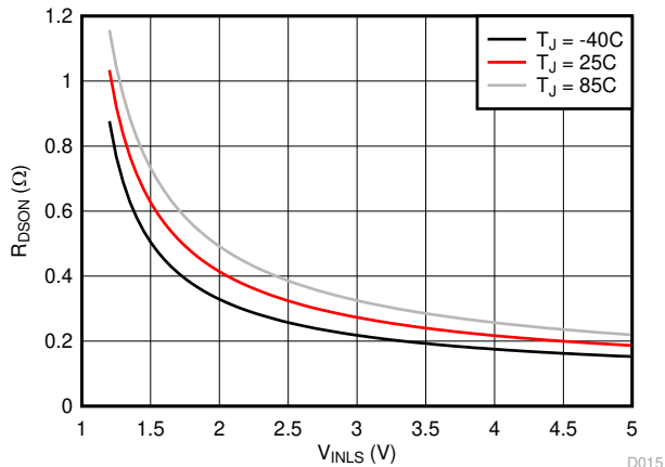
Figure 8-5. LS/LDO Switch On Resistance vs. VINLS
