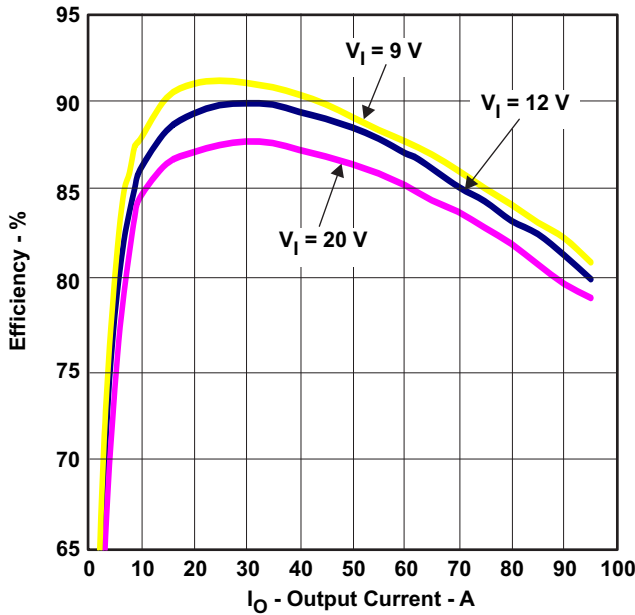
Figure 20. CPU3 Efficiency
