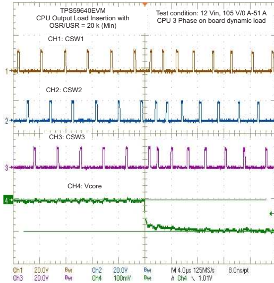
Figure 28. CPU3 Output Load Insertion With OSR/USR = 20k (Min)
