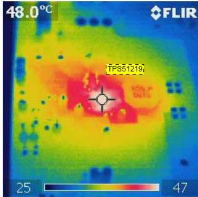
Figure 82. TPS51219 Thermal
