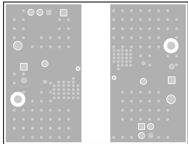
Figure 4-4. Ground Layer 2
