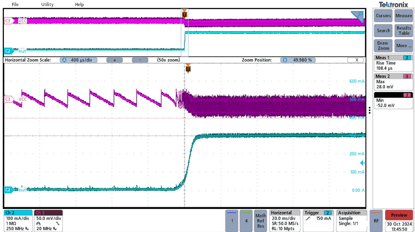
Figure 3-10. Load transient, VINP=5.0V, VCC=5.0V, No load ( I_{out} =0mA) to Full load ( I_{out} =300mA)
