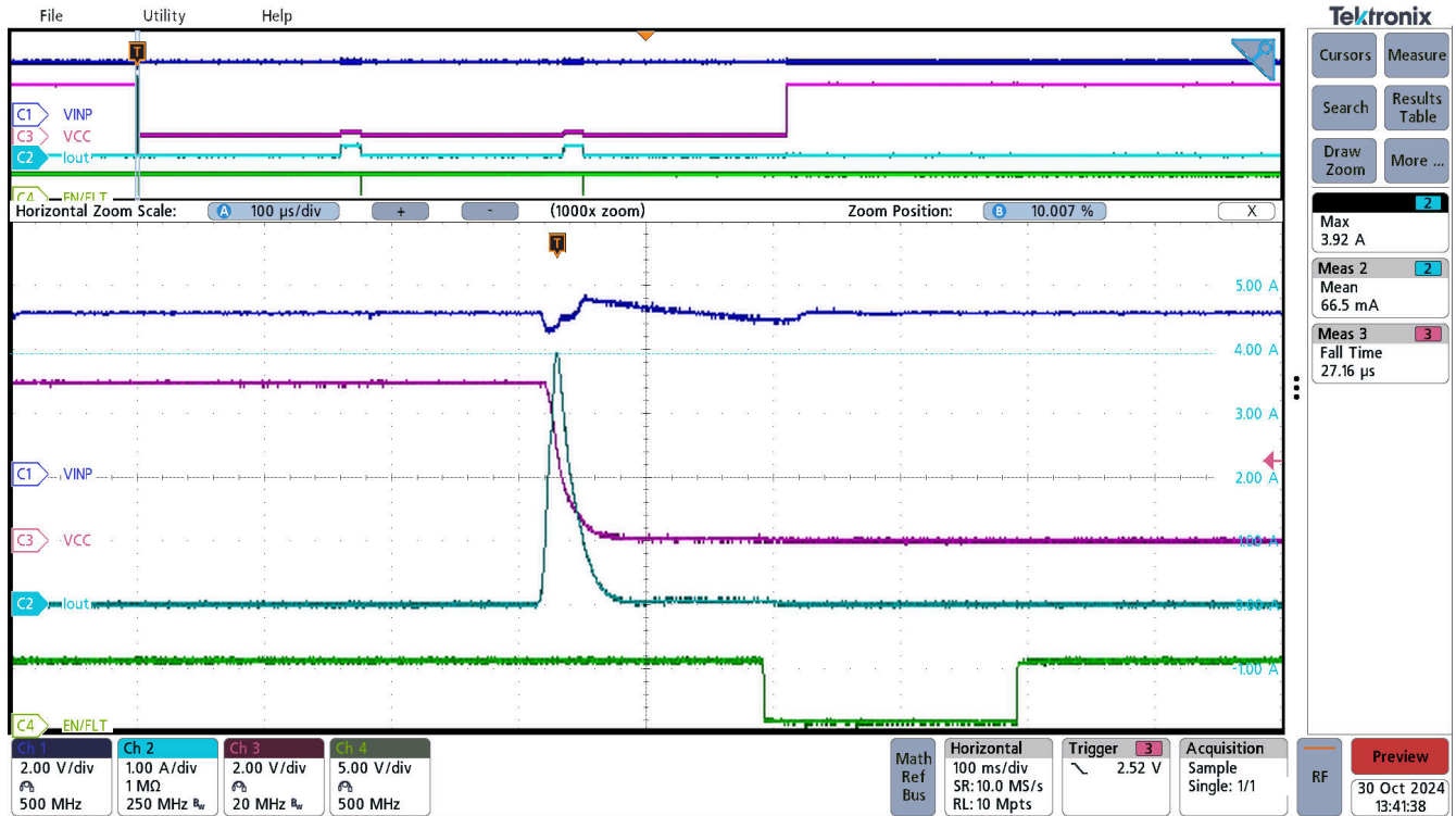
Figure 3-12. Short circuit, VINP=5.0V, VCC=5.0V
