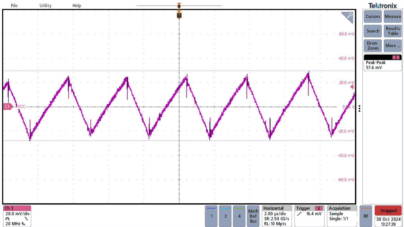
Figure 3-9. VCC AC Ripple, VINP=5.0V, VCC=5.0V, I out =300mA
