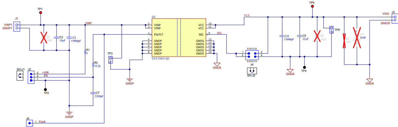
Figure 3-1. Schematic
