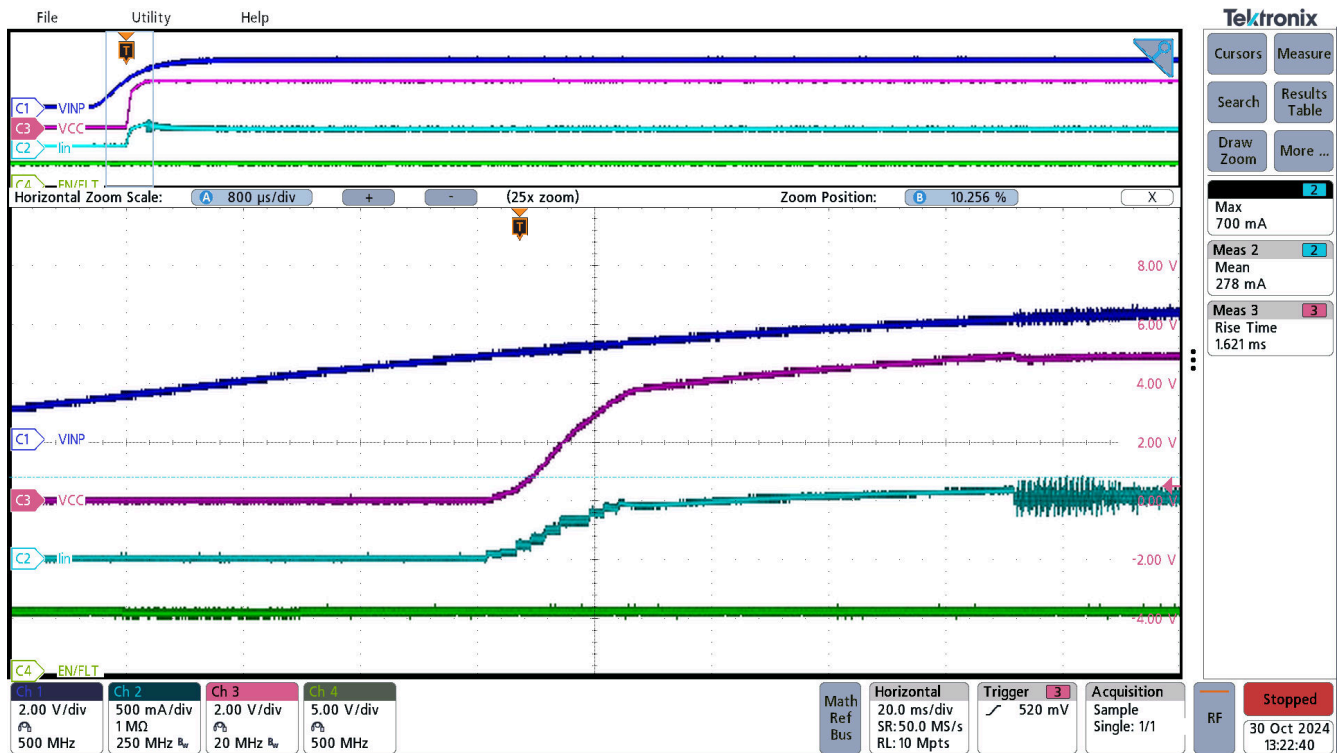
Figure 3-5. Start-up, sequence EN=5.0V → VINP=5.0V, VCC=5.0V, R load =18Ω
