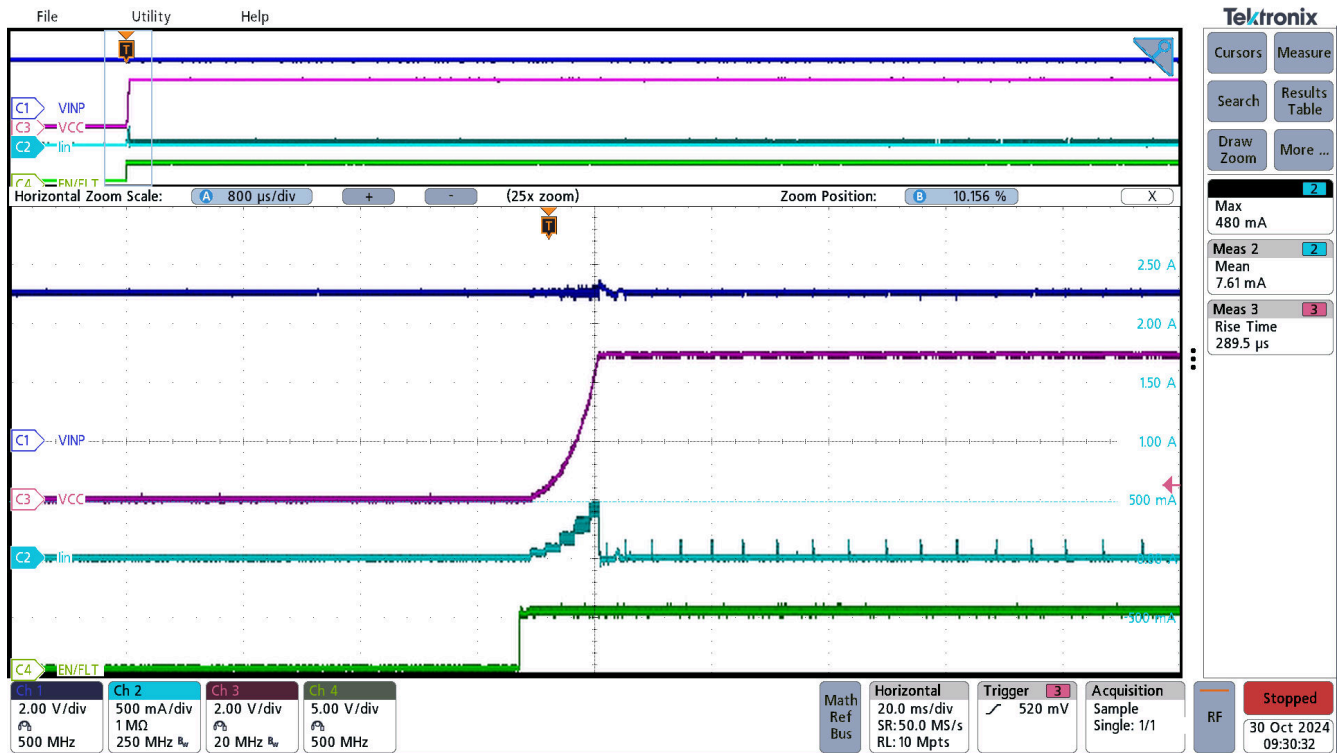
Figure 3-6. Inrush current , sequence VINP=5.0V \rightarrow EN=5.0V, VCC=5.0V, I out =0mA, Toggling EN
