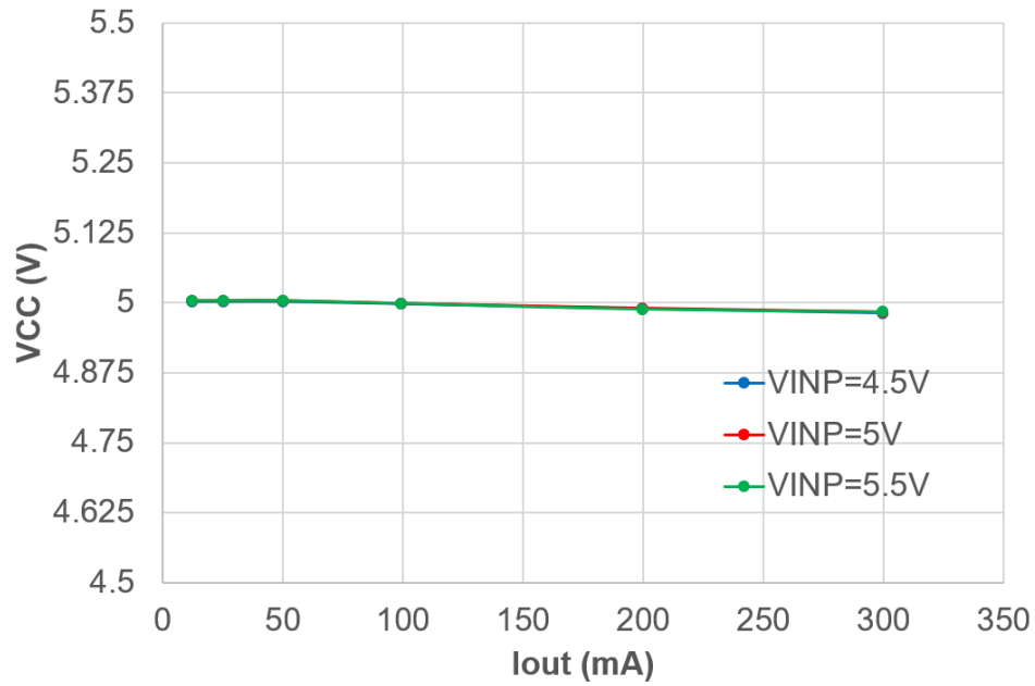
Figure 3-3. Regulation vs Load Current
