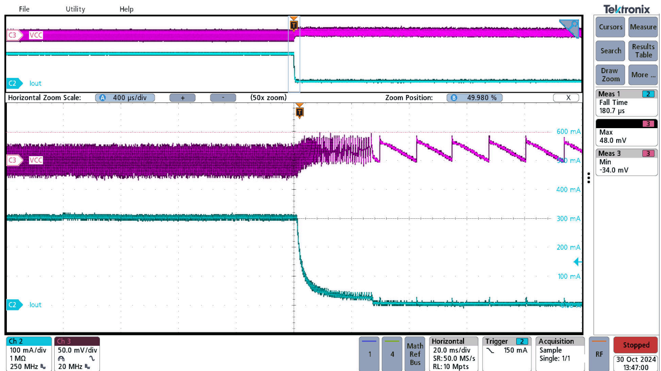
Figure 3-11. Load transient, VINP=5.0V, VCC=5.0V, Full load ( I_{out} =300mA) to No load ( I_{out} =0mA)
