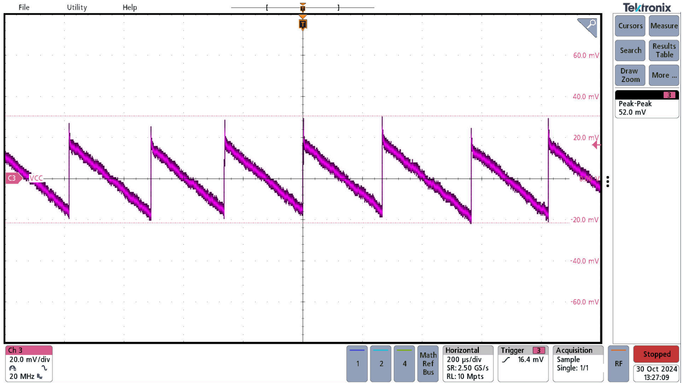
Figure 3-8. VCC AC Ripple, VINP=5.0V, VCC=5.0V, I out =0mA
