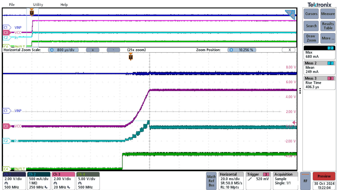
Figure 3-7. Inrush current, sequence VINP=5.0V \rightarrow EN=5.0V, VCC=5.0V, R load =18 \Omega , Toggling EN
