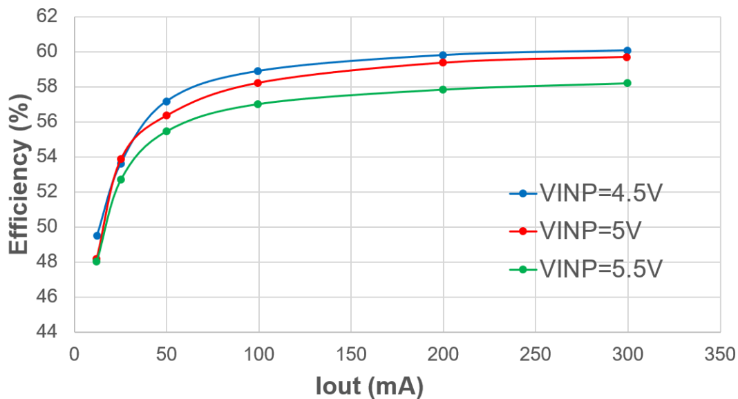
Figure 3-2. Efficiency
