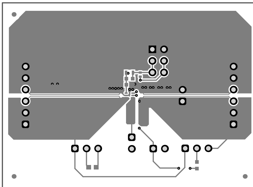
Figure 3-3. Top Layer
