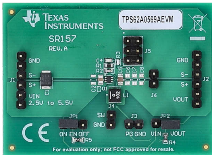
TPS62A0569AEVM-157
