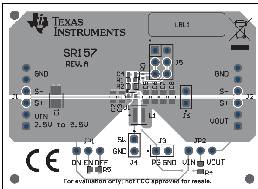
Figure 3-2. Mask (Top View)
