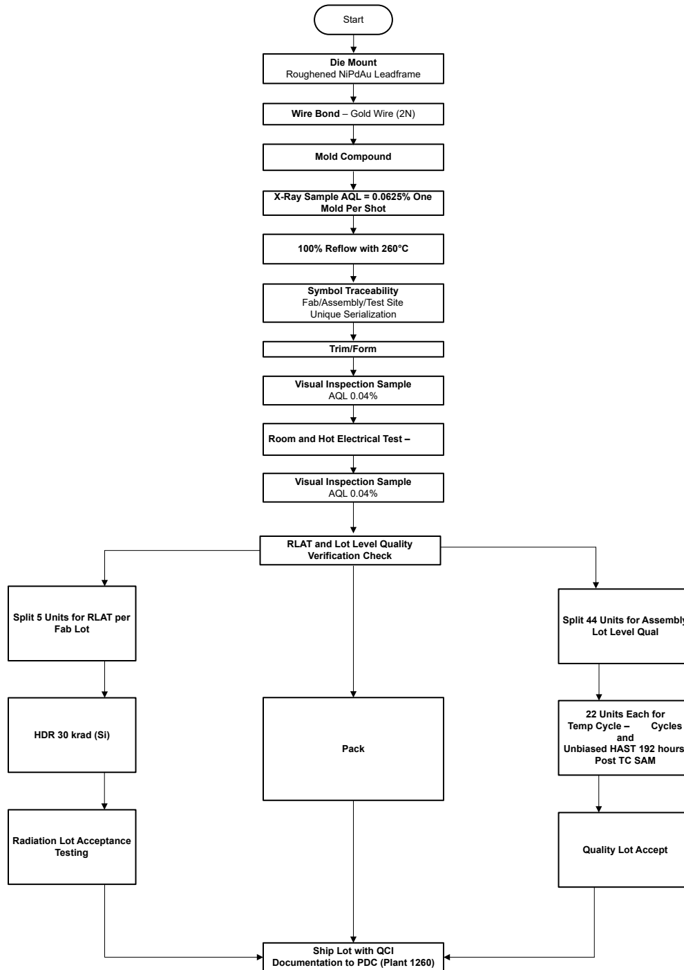
Figure 1-1. INA951-SEP Space Enhanced Plastic Production Flow Chart
