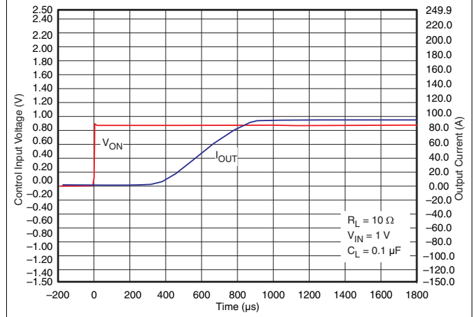
Figure 41. t_{ON} Response
