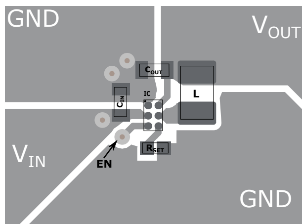
Figure 62. Recommended PCB Layout YBG Package
