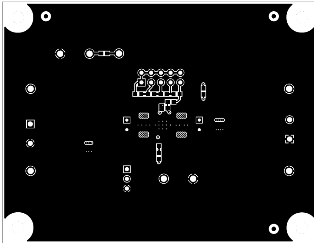
Figure 4-5. Bottom Layer
