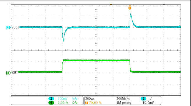
Figure 3-4. Transient Performance
