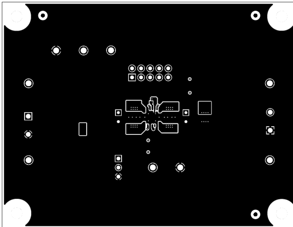
Figure 4-2. Top Copper Layer
