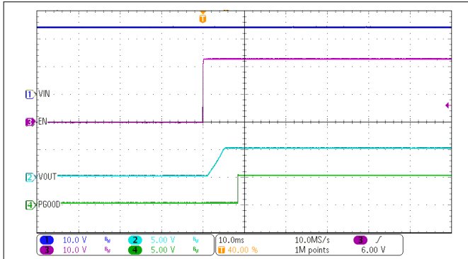
Figure 3-1. ENABLE Start-Up Waveform
