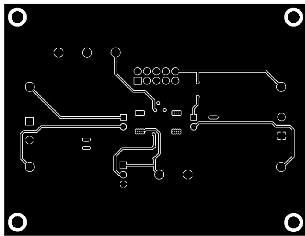
Figure 4-4. Signal Layer 2
