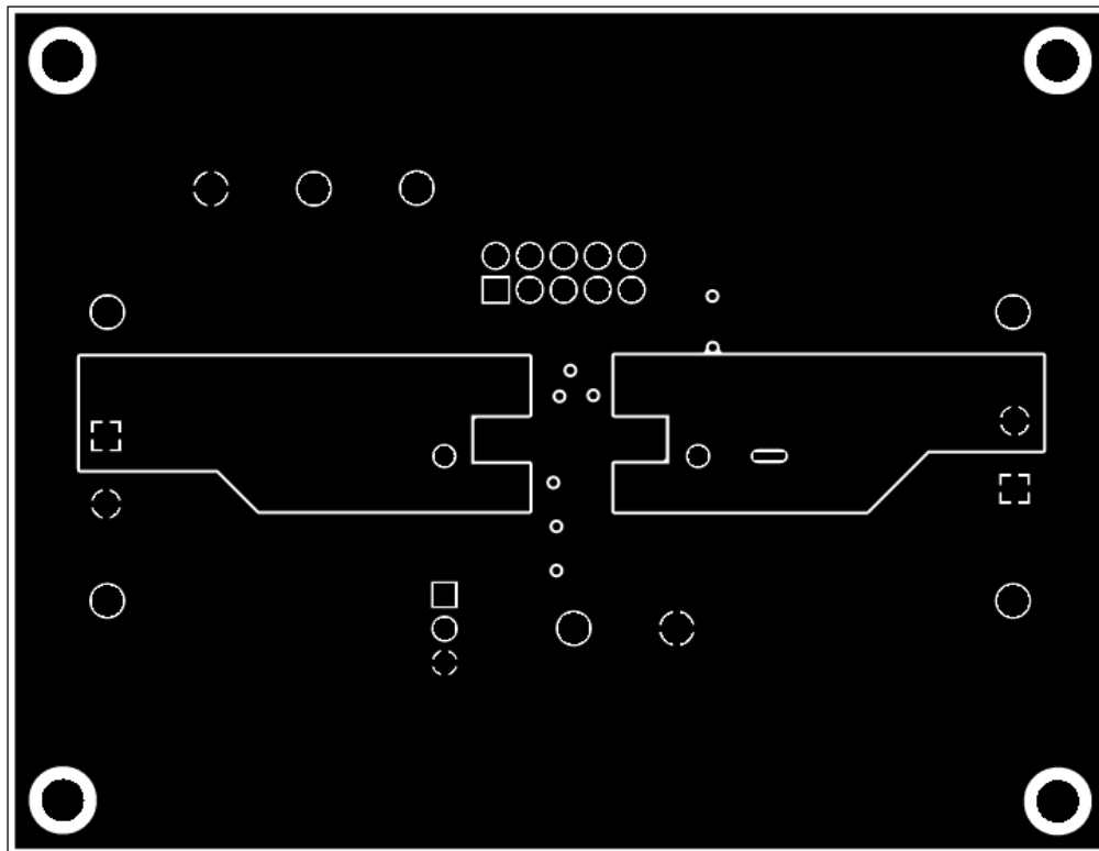
Figure 4-3. Signal Layer 1
