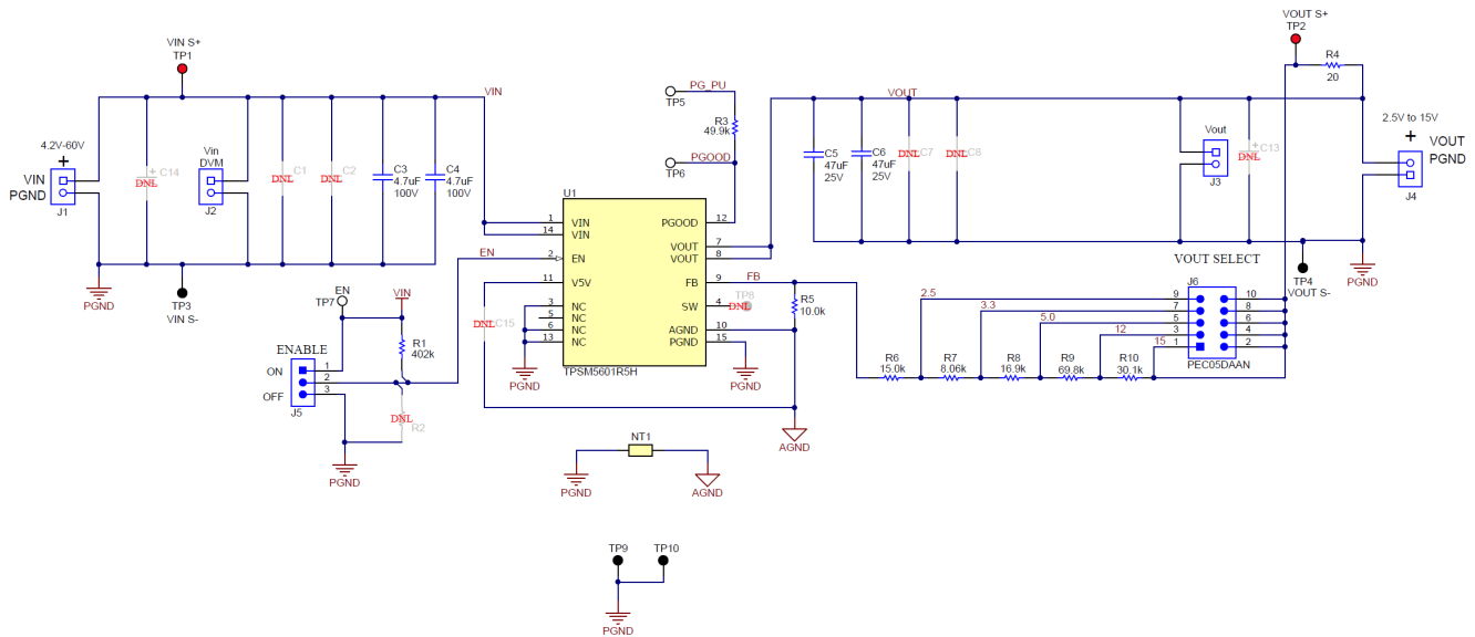
Figure 5-1. TPSM5601R5HEVM Schematic
