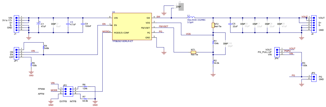
Figure 7-1. TPS629210EEVM Schematic
