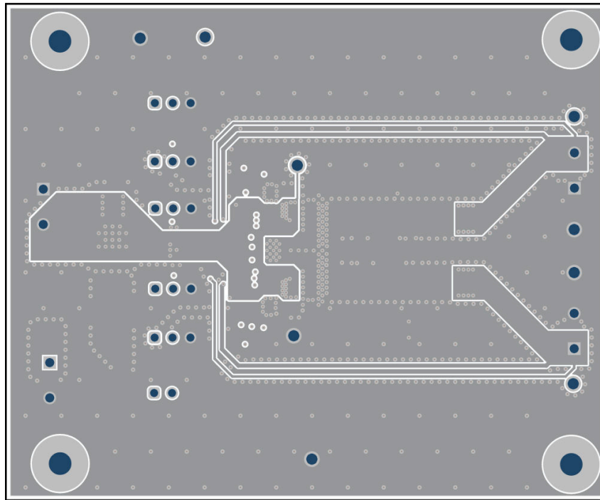
Figure 6-6. Layer 3 Copper
