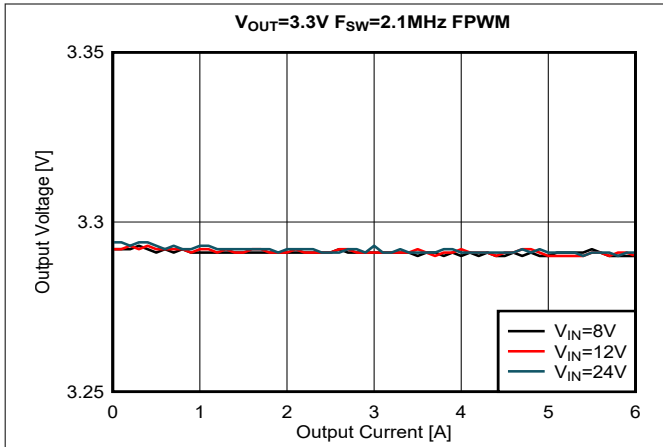
Figure 5-7. Load Regulation, V OUT = 3.3 V, FPWM Mode
