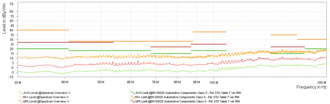
Figure 5-25. CISPR 25 Radiated Emissions: 30 MHz to 200 MHz, BICON
