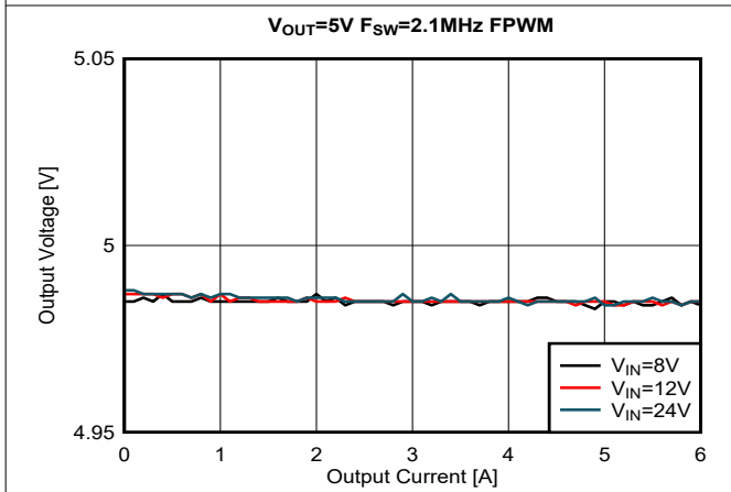
Figure 5-9. Load Regulation, V OUT = 5.0 V, FPWM Mode
