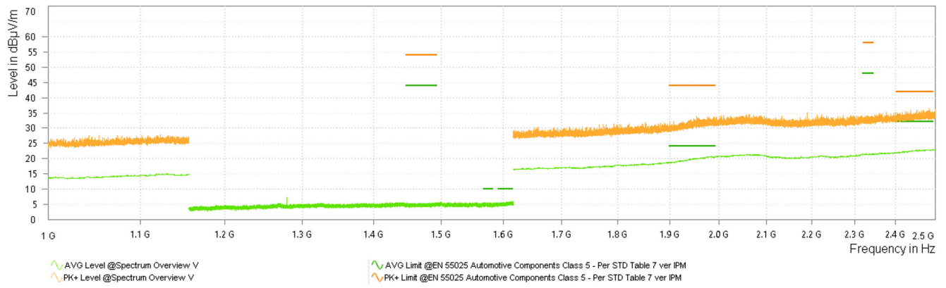
Figure 5-27. CISPR 25 Radiated Emissions: 1 GHz to 2.5G Hz, HORN
