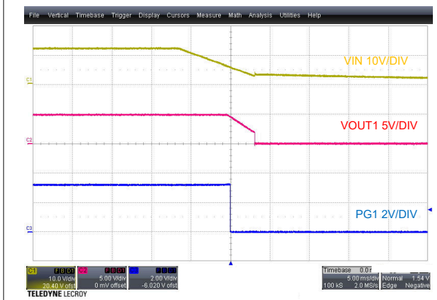
Figure 5-13. Shutdown, VOUT1 = 5.0 V
