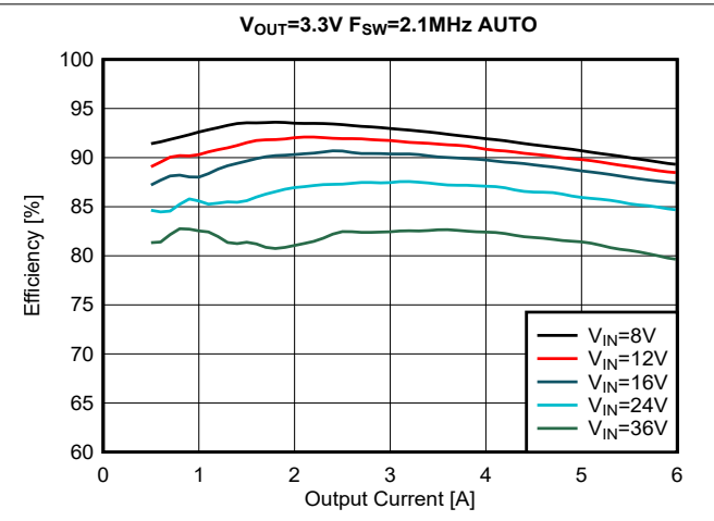
Figure 5-2. Efficiency, V_{OUT} = 3.3\text{ V} , AUTO Mode
