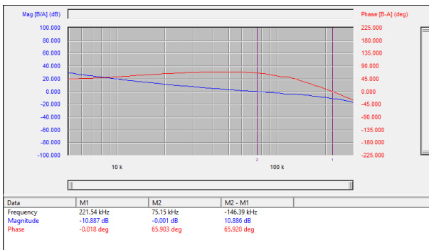
Figure 5-19. Bode Plot (CH1)
