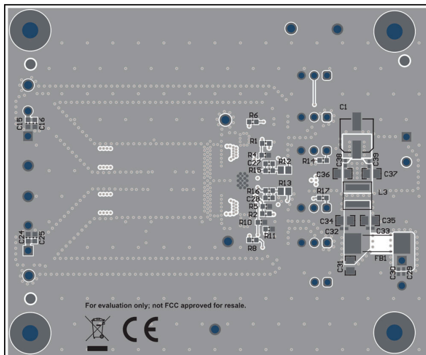
Figure 6-3. Bottom Component View
