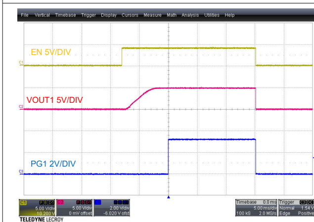
Figure 5-15. Enable ON and OFF, VOUT1 = 5.0 V
