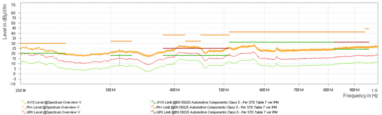
Figure 5-26. CISPR 25 Radiated Emissions: 200 MHz to 1 GHz, LOG
