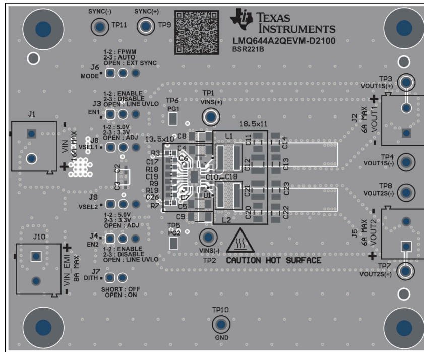
Figure 6-2. Top Component View
