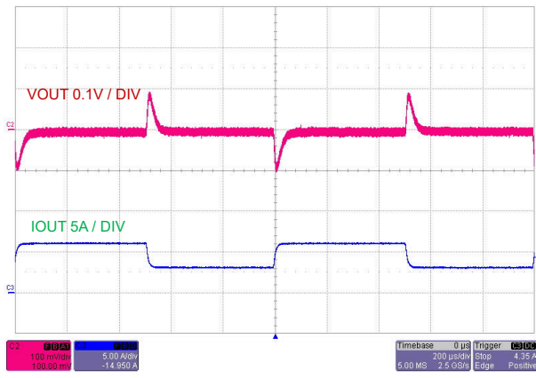
Figure 5-17. Load Transient (CH1), IOUT1 = 3 A to 6 A A
