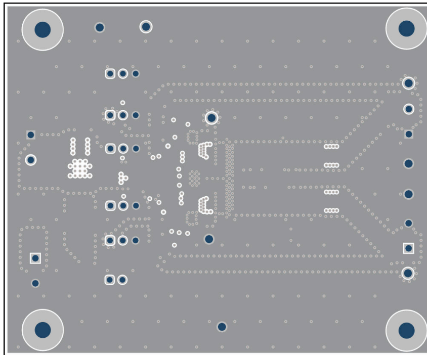
Figure 6-5. Layer 2 Copper
