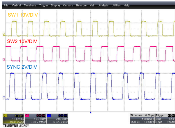
Figure 5-21. SYNC and Interleaving, VOUT1 = 3.3 V, VOUT2 = 5.0 V
