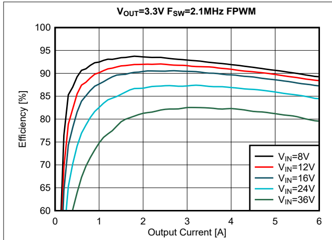
Figure 5-1. Efficiency, V_{OUT} = 3.3\text{ V} , FPWM Mode
