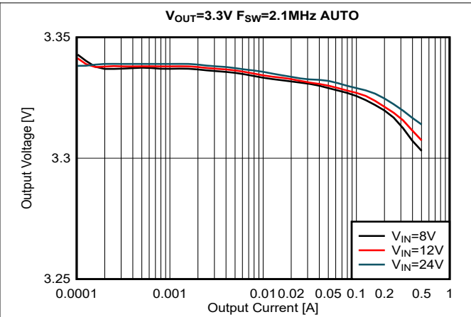
Figure 5-8. Load Regulation, V OUT = 3.3 V, AUTO Mode
