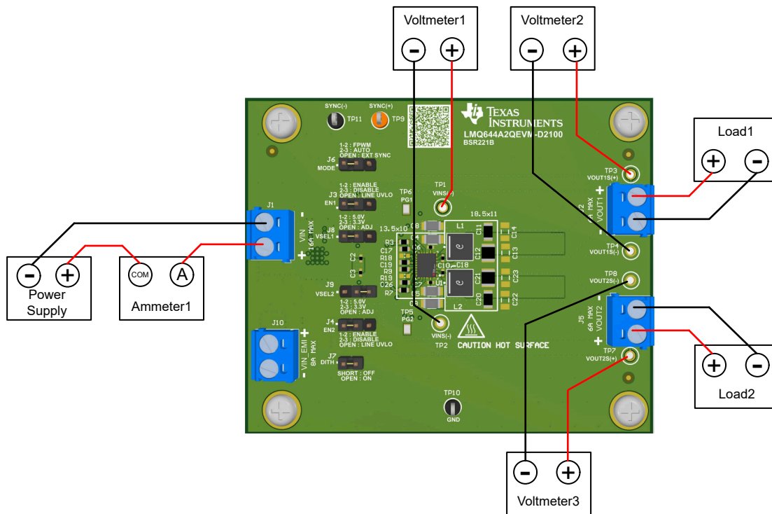
Figure 4-1. EVM Test Setup
