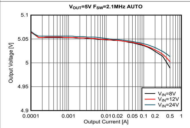
Figure 5-10. Load Regulation, V OUT = 5.0 V, AUTO Mode
