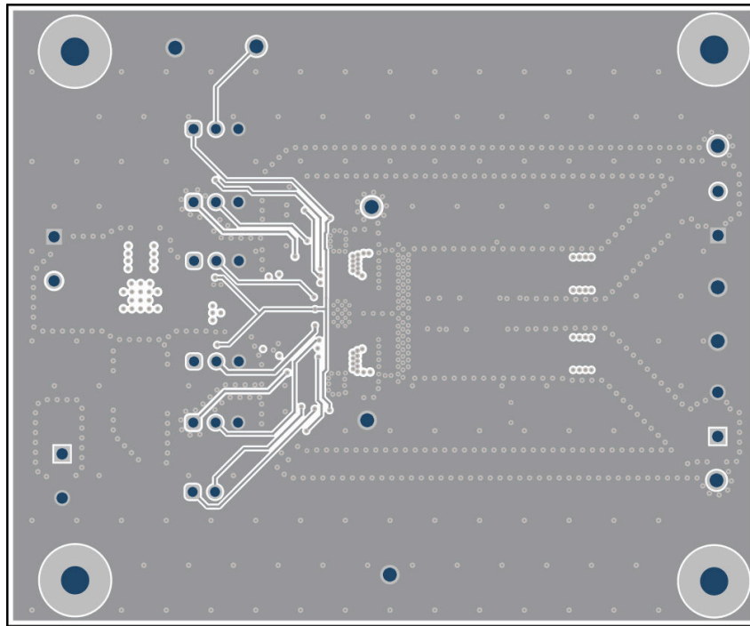
Figure 6-8. Layer 5 Copper
