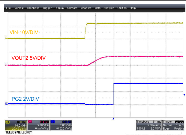
Figure 5-12. Start-Up, VOUT2 = 3.3 V
