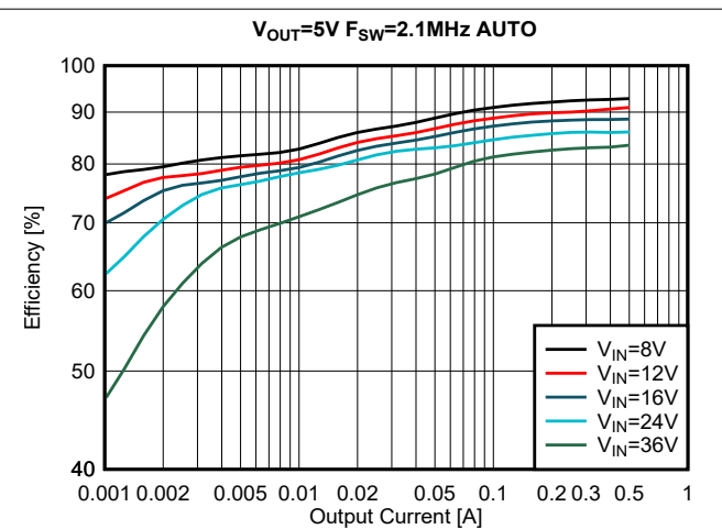
Figure 5-6. Efficiency, V_{OUT} = 5.0\text{ V} , AUTO Mode
