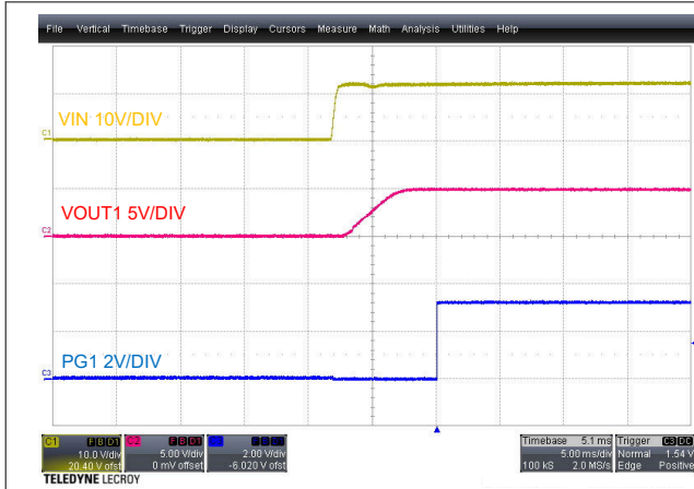
Figure 5-11. Start-Up, VOUT1 = 5.0 V
