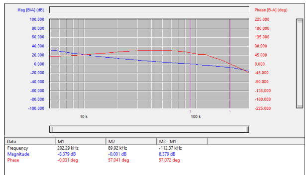
Figure 5-20. Bode Plot (CH2)
