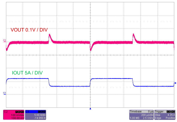
Figure 5-18. Load Transient (CH2), IOUT2 = 3 A to 6 A A
