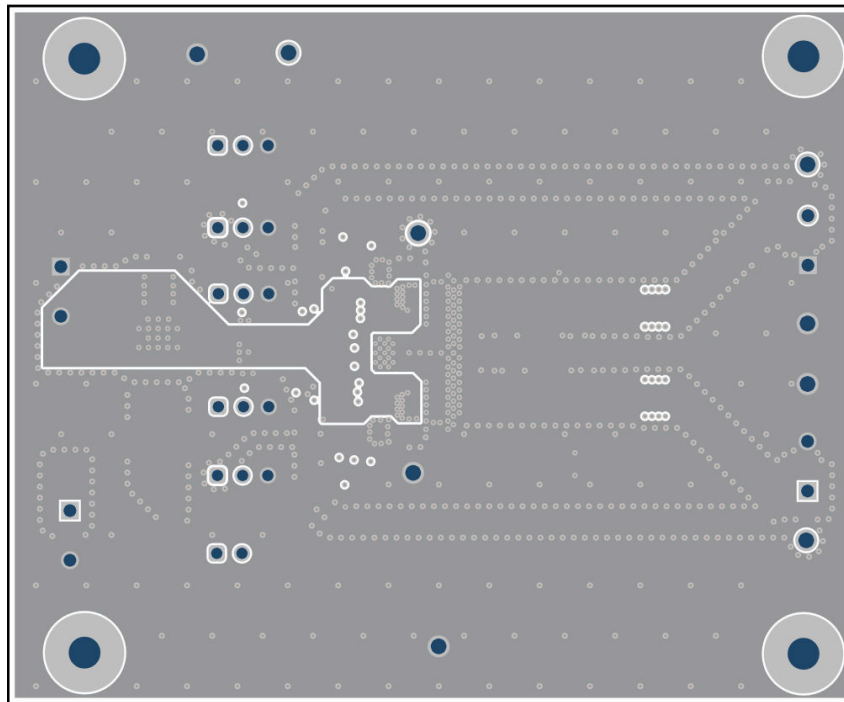
Figure 6-7. Layer 4 Copper
