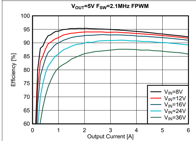
Figure 5-3. Efficiency, V_{OUT} = 5.0\text{ V} , FPWM Mode
