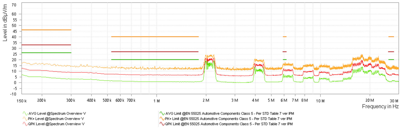
Figure 5-24. CISPR 25 Radiated Emissions: 150 kHz to 30 MHz, MONOPOLE
