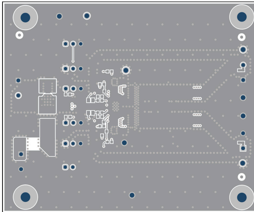
Figure 6-9. Bottom Layer Copper (Viewed From Top)
