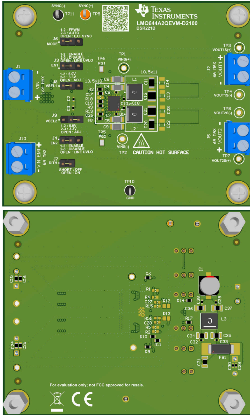
Figure 3-1. LMQ644A2QEVM-D2100 EVM Photo
