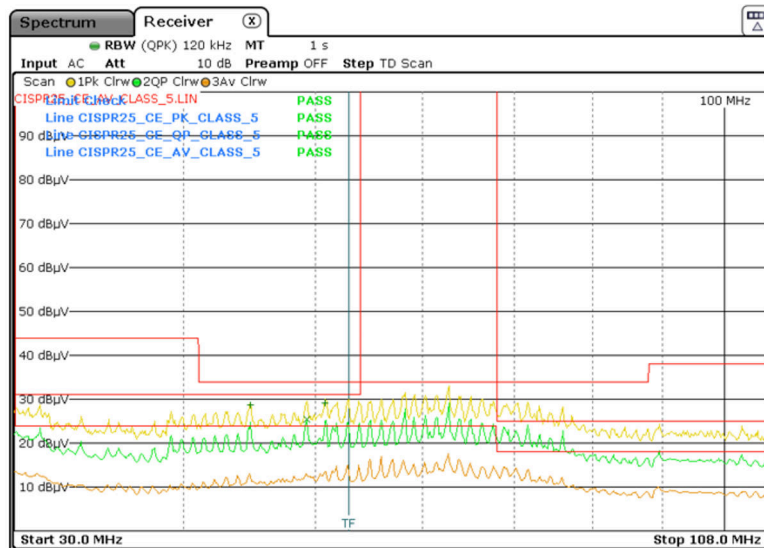
Figure 5-23. CISPR 25 Conducted Emissions: 30 MHz to 108 MHz
