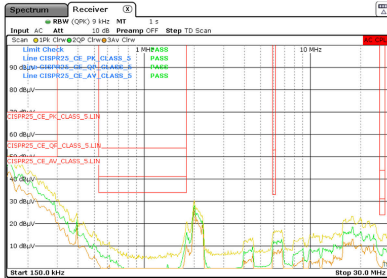
Figure 5-22. CISPR 25 Conducted Emissions: 150 kHz to 30 MHz
