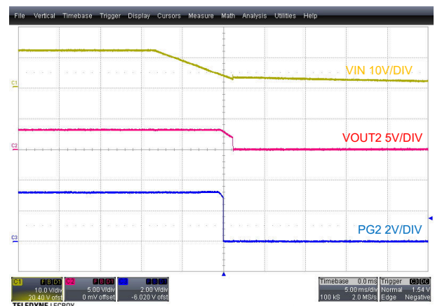
Figure 5-14. Shutdown, VOUT2 = 3.3 V
