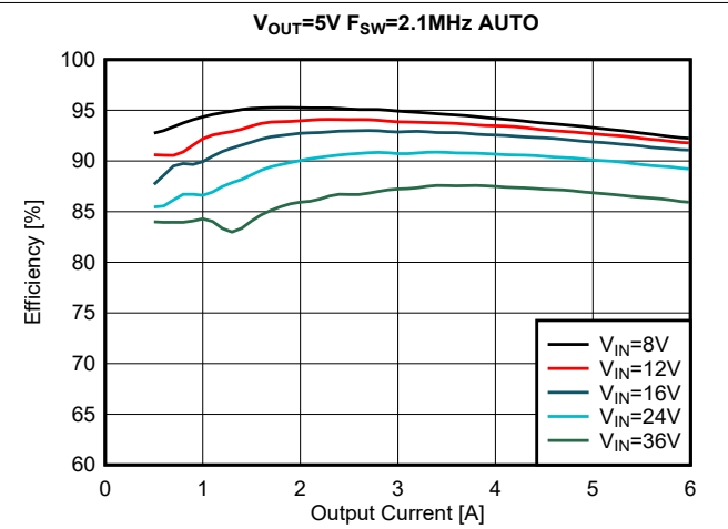
Figure 5-4. Efficiency, V_{OUT} = 5.0\text{ V} , AUTO Mode
