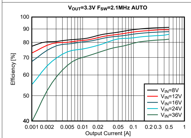
Figure 5-5. Efficiency, V_{OUT} = 3.3\text{ V} , AUTO Mode
