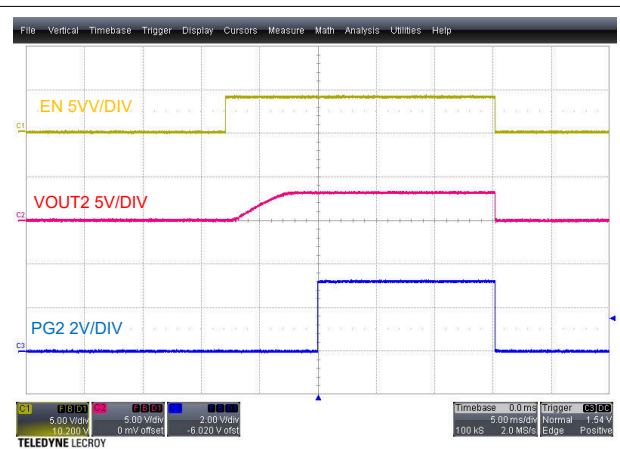
Figure 5-16. Enable ON and OFF, VOUT2 = 3.3 V
