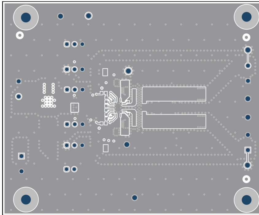
Figure 6-4. Top Layer Copper
