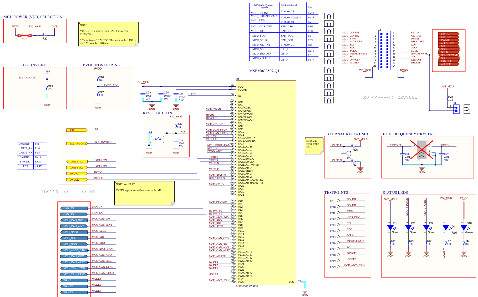
Figure 4-2. MCU MSPM0G3507-Q1
