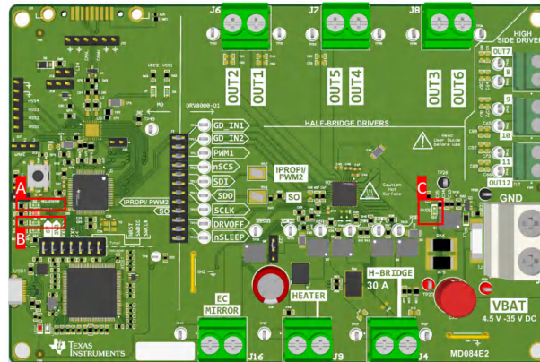
Figure 2-4. LED Indicators
