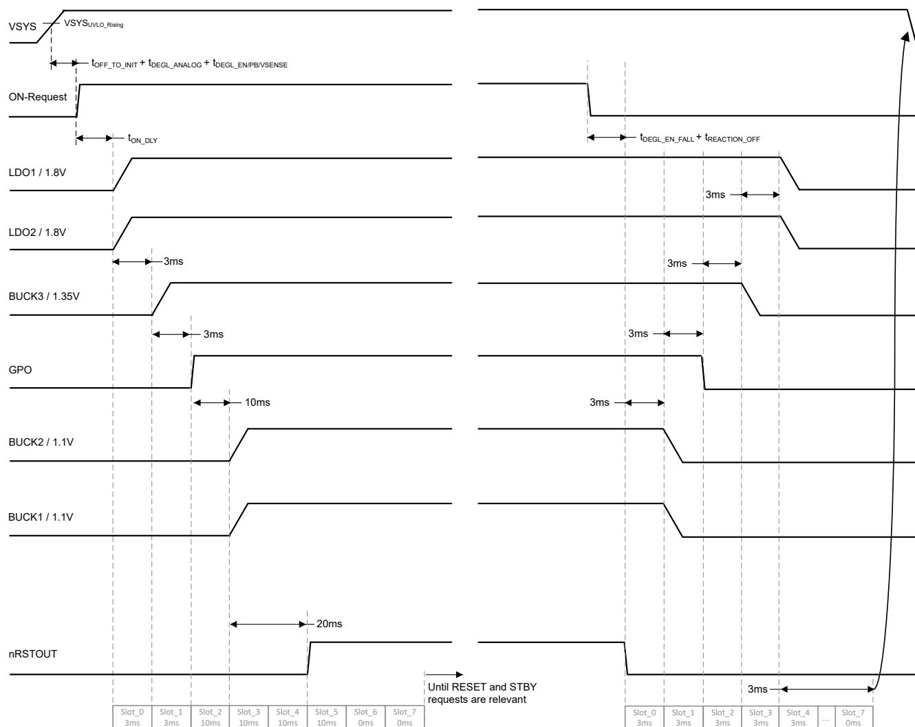
Figure 2-1. TPS6521403 Power Sequence
