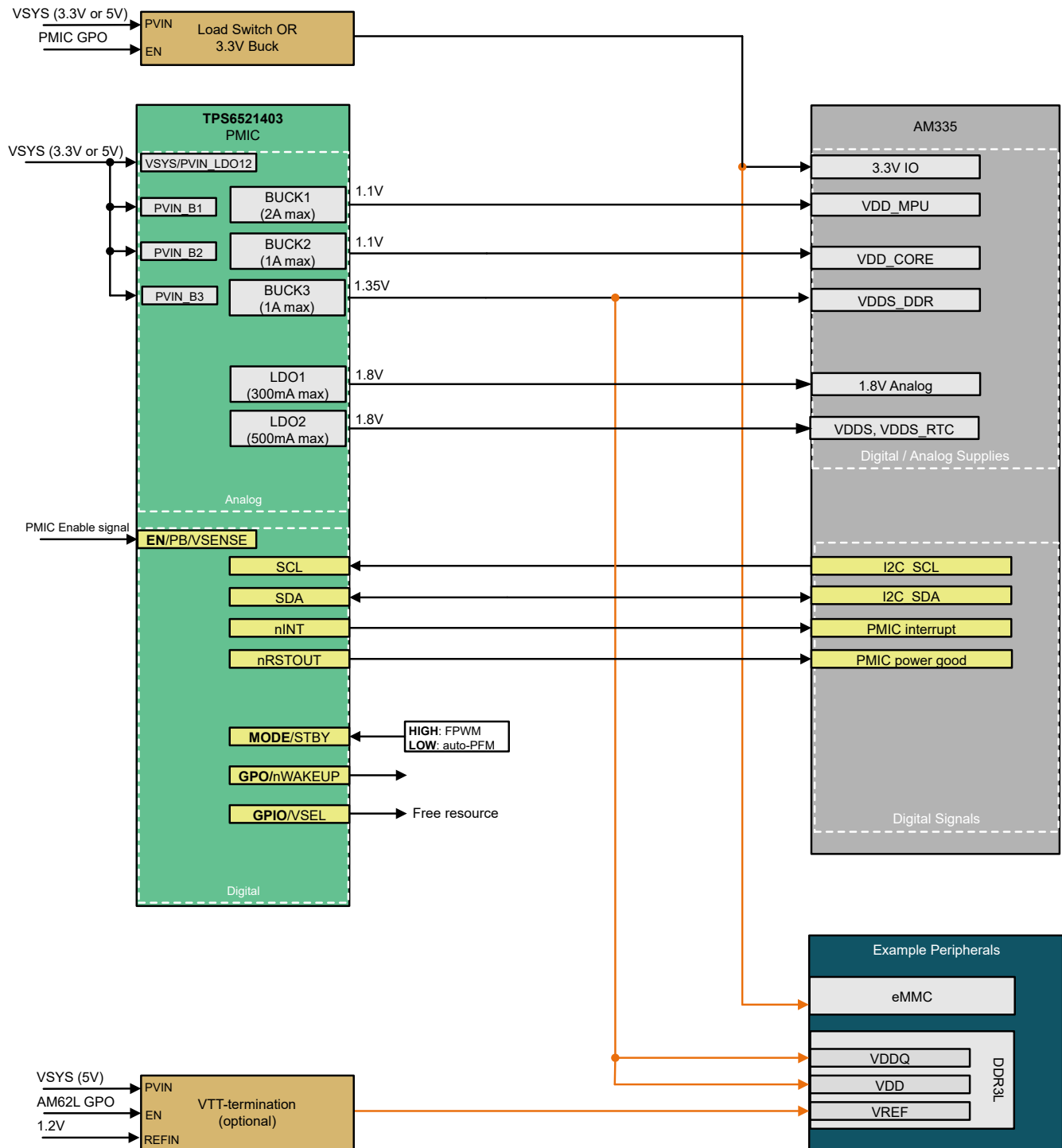
Figure 2-2. TPS6521403 Example Block Diagram
