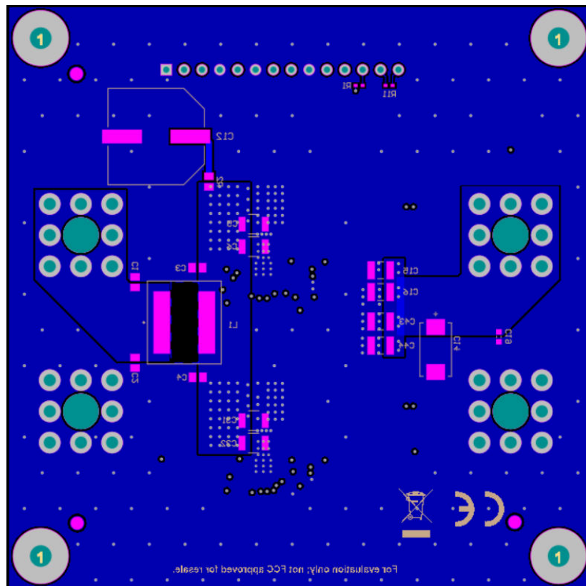
Figure 4-7. Bottom Copper (Top View)
