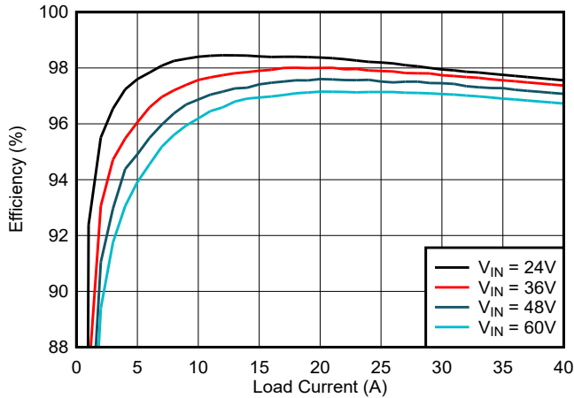
Figure 3-1. Efficiency, V_{OUT} = 12V , FPWM/SYNC Tied High
