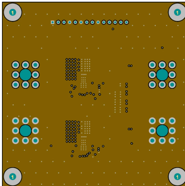
Figure 4-3. Layer 2 Copper (Top View)
