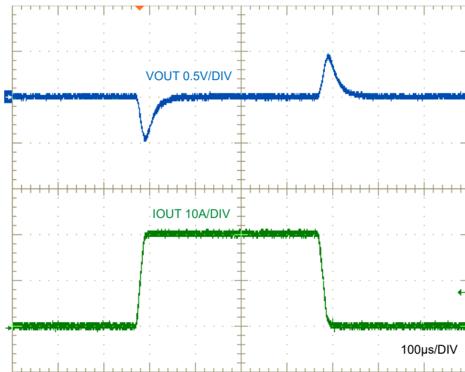
Figure 3-4. Load Transient Response, V_{IN} = 48V , FPWM, 0A to 20A at 1A/ \mu s
