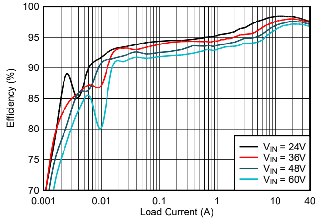
Figure 3-2. Efficiency, V_{OUT} = 12V , FPWM/SYNC Tied Low
