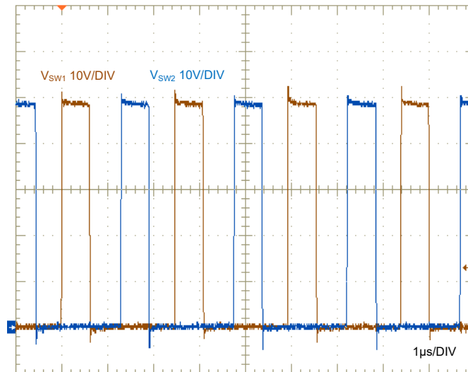
Figure 3-8. Switch-node Voltages, V_{IN} = 48V , I_{OUT} = 20A
