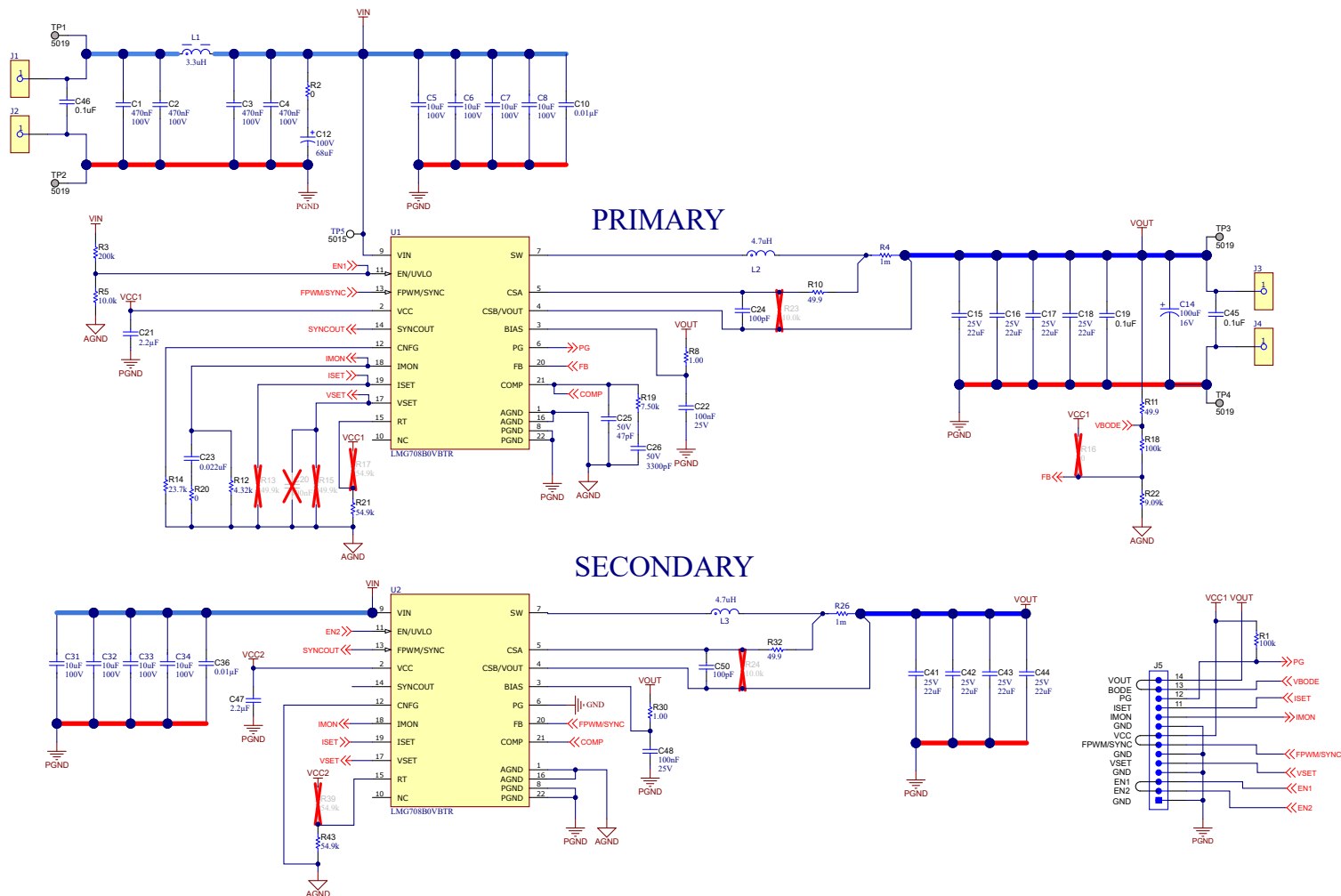
Figure 4-1. Two-phase EVM Schematic
