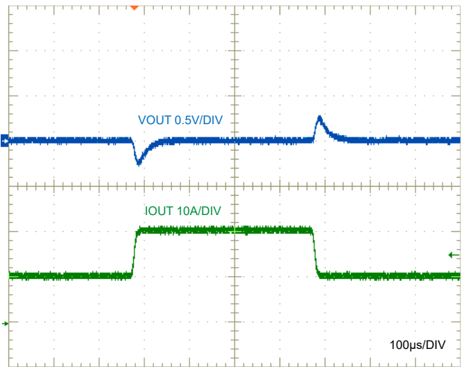
Figure 3-5. Load Transient Response, V_{IN} = 48V , FPWM, 10A to 20A at 1A/ \mu s
