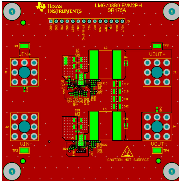
Figure 4-2. Top Copper (Top View)
