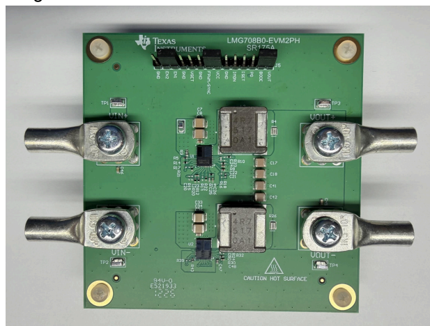
LMG708B0 Two-Phase EVM, 84mm × 84mm (3.3" × 3.3")
