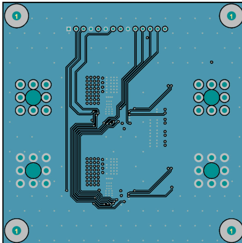
Figure 4-4. Layer 3 Copper (Top View)
