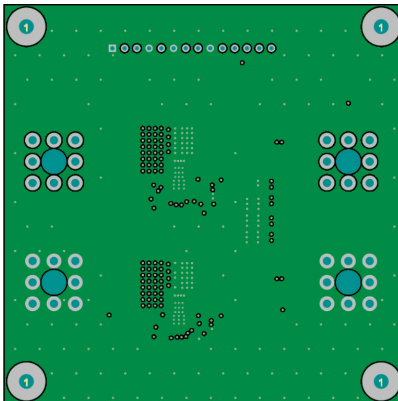
Figure 4-5. Layer 4 Copper (Top View)
