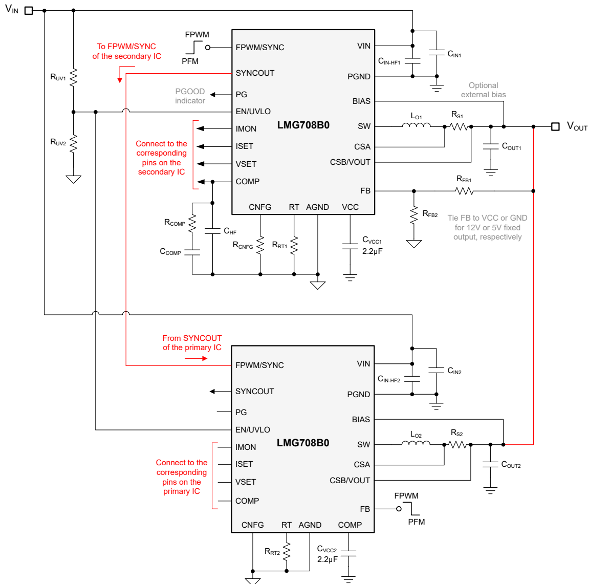
Figure 1-1. LMG708B0 Two-Phase GaN Synchronous Buck Regulator Simplified Schematic
