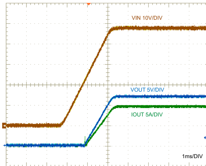
Figure 3-6. Start-Up Characteristic, V_{IN} Ramped to 48V, I_{OUT} = 10A Resistive
