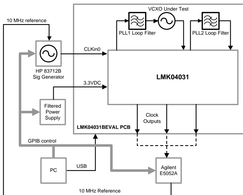
Figure 4. Phase Noise and Jitter Measurement Test Setup
