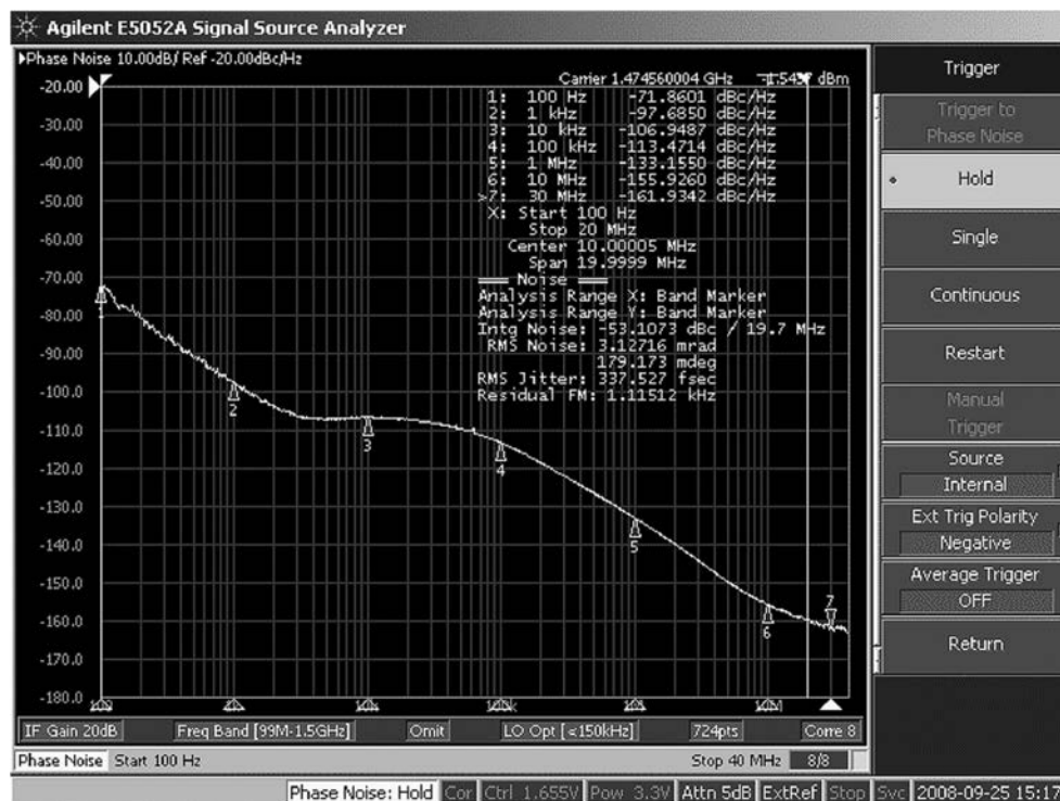
Figure 21. LMK04031 Four Phase Noise, Crystek CVPD-920-61.44 VCXO
