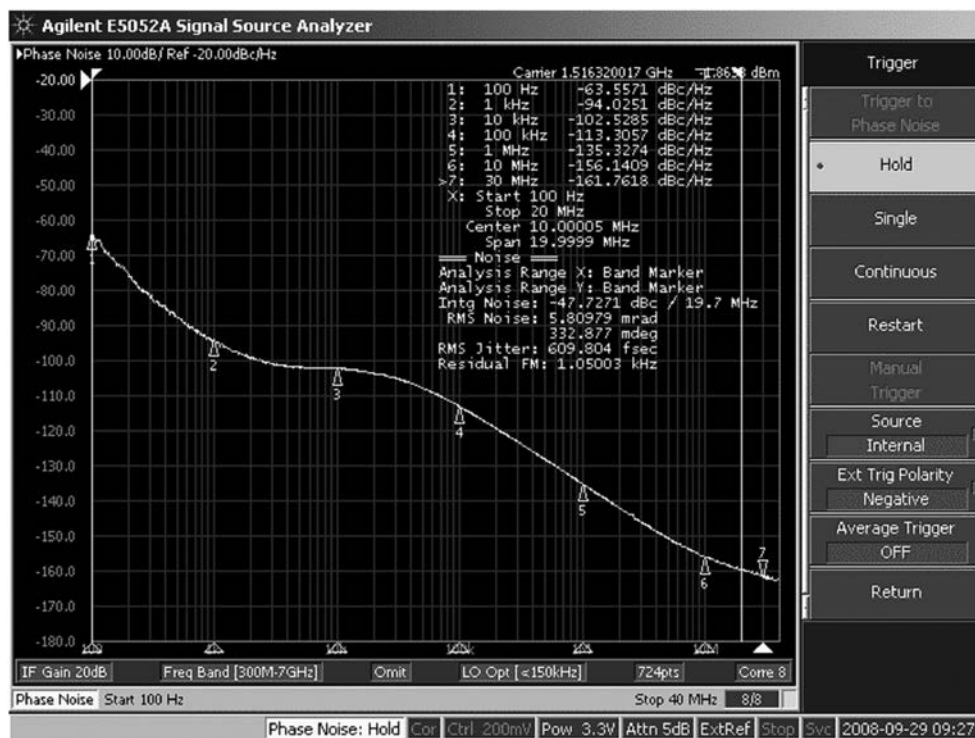
Figure 31. LMK04031 Four Phase Noise, Epson Toyocom VG-4231 VCXO
