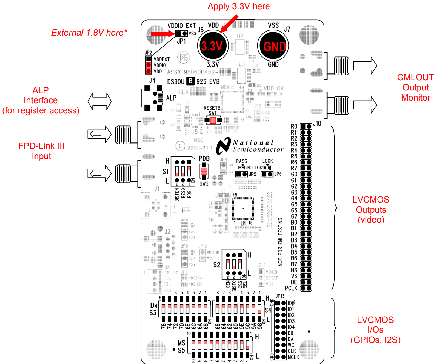
Figure 1: DS90UB926Q EVB
