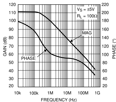
Figure 5-16. Transimpedance
