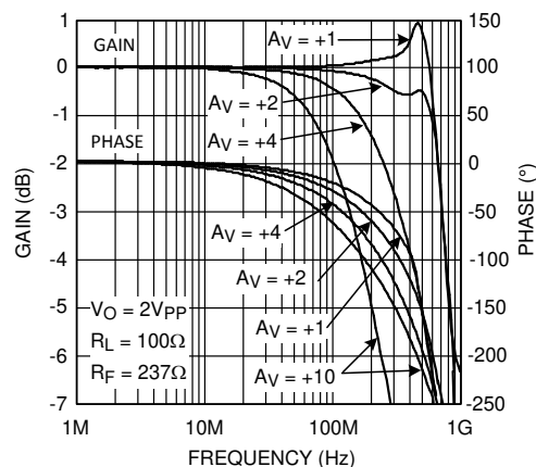
Figure 5-2. Noninverting Frequency Response
