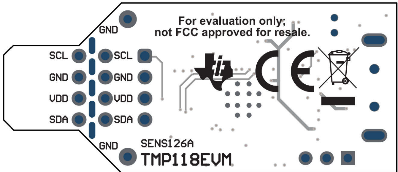
Figure 4-2. PCB Top
