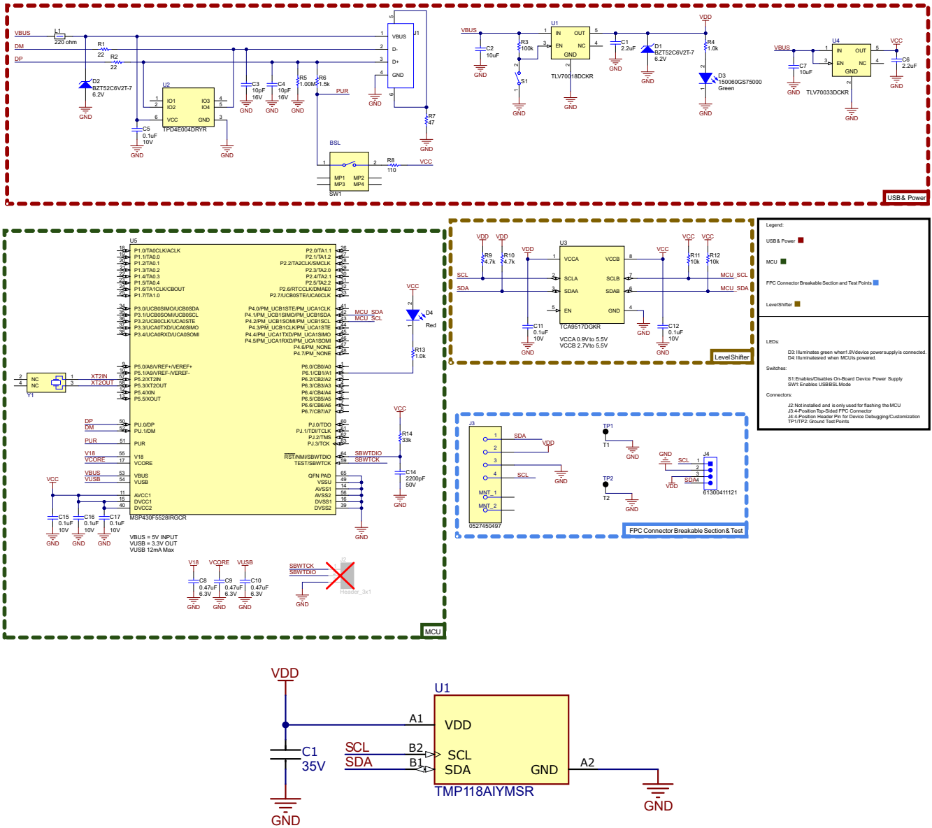
Figure 4-1. Schematic
