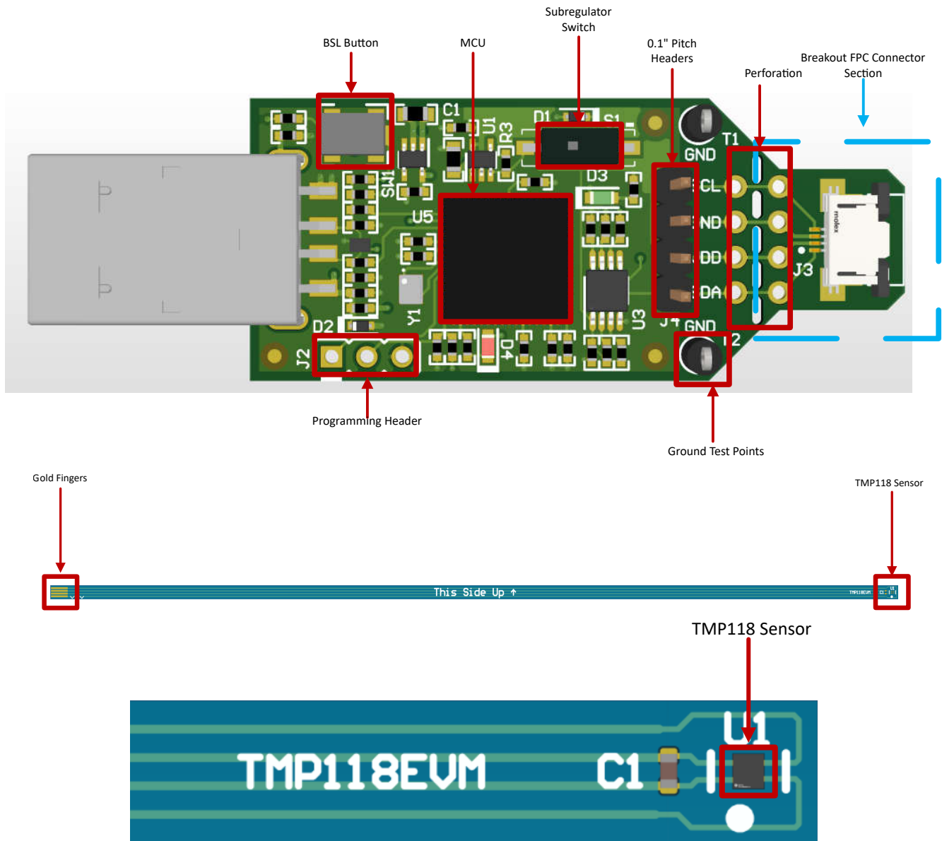
Figure 2-1. TMP118EVM Board Sections
