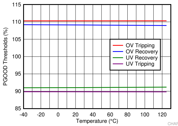
Figure 6-9. PGOOD Thresholds
