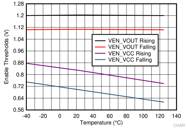
Figure 6-8. Enable Thresholds
