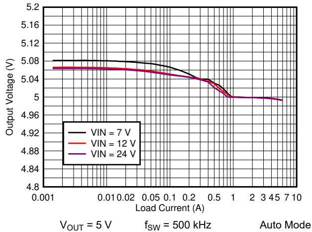
Figure 8-9. TPS7H4010-SEP Load and Line Regulation
