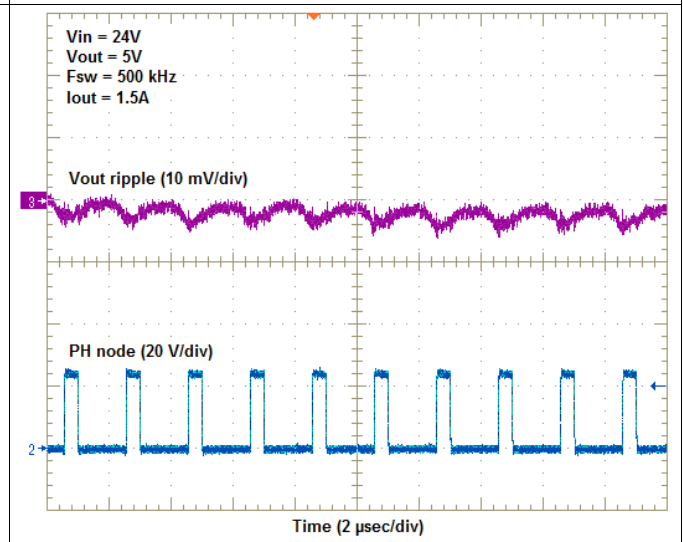
Figure 5. LMZ36002EVM Ripple Voltage (Fsw = 500 KHz)
