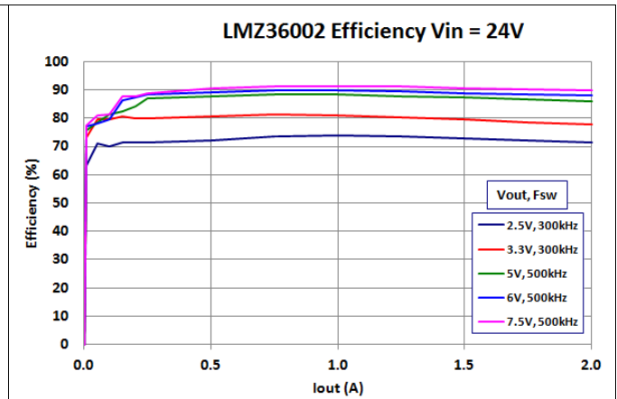
Figure 3. LMZ36002EVM Efficiency (Vin = 24V)
