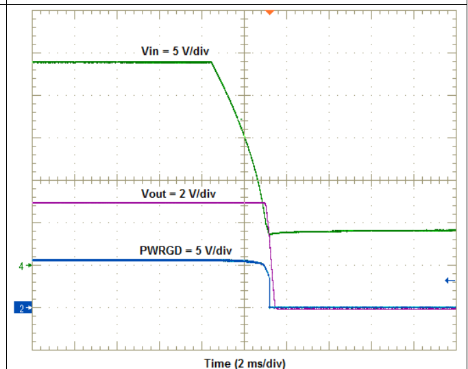
Figure 7. LMZ36002EVM Shut-down Waveforms
