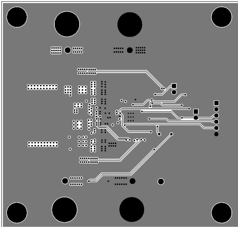
Figure 17. Mid Layer 3
