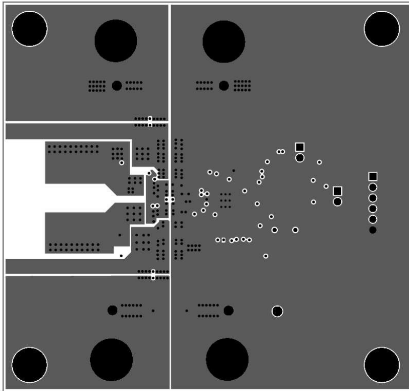
Figure 16. Mid Layer 2
