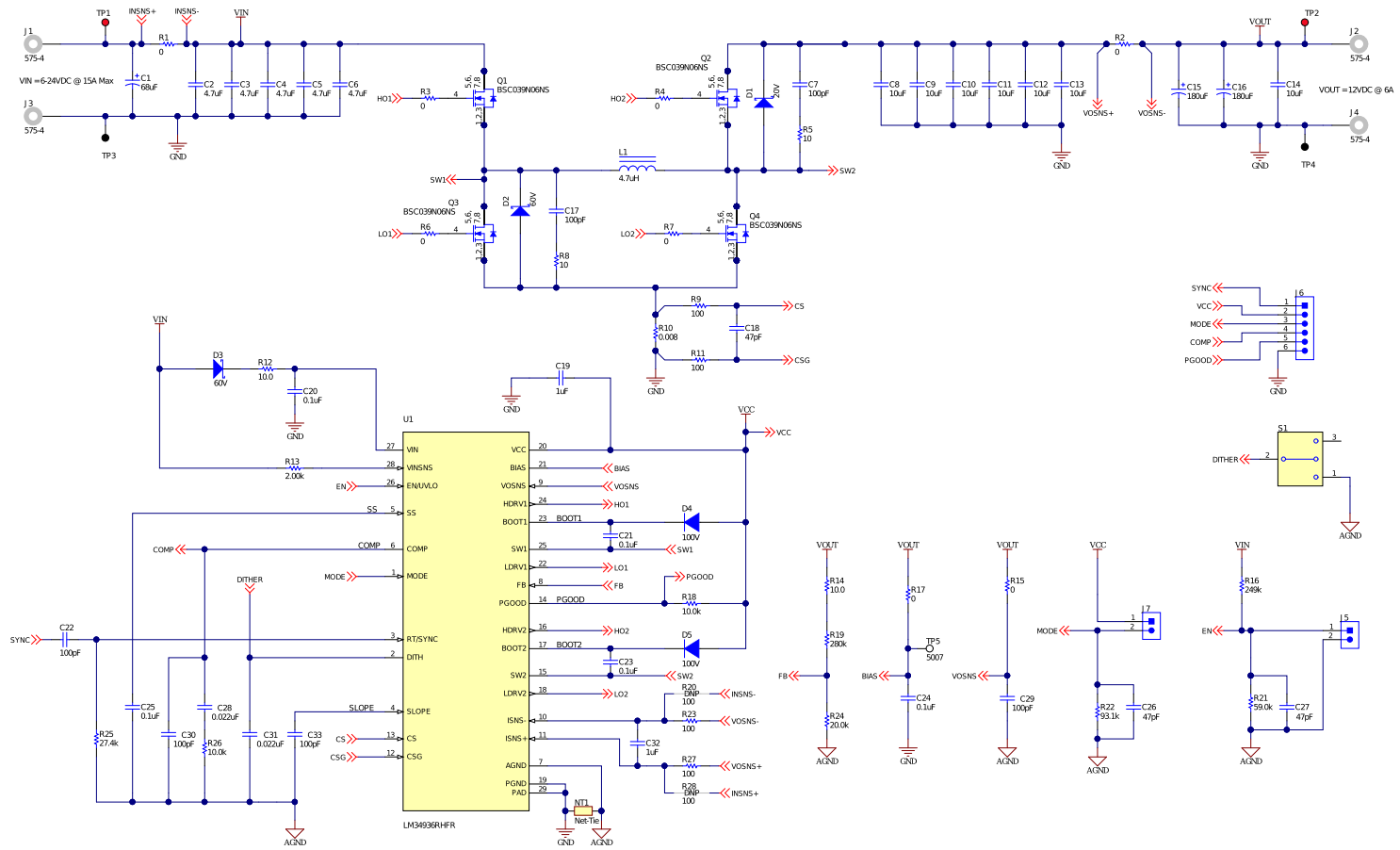
Figure 12. LM34936EVM Schematic
