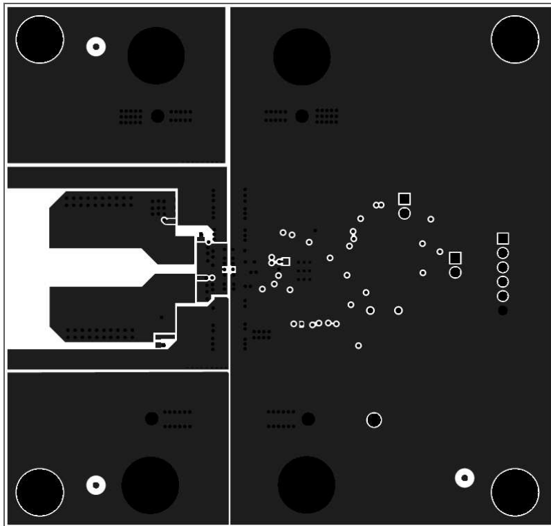
Figure 14. Top Layer
