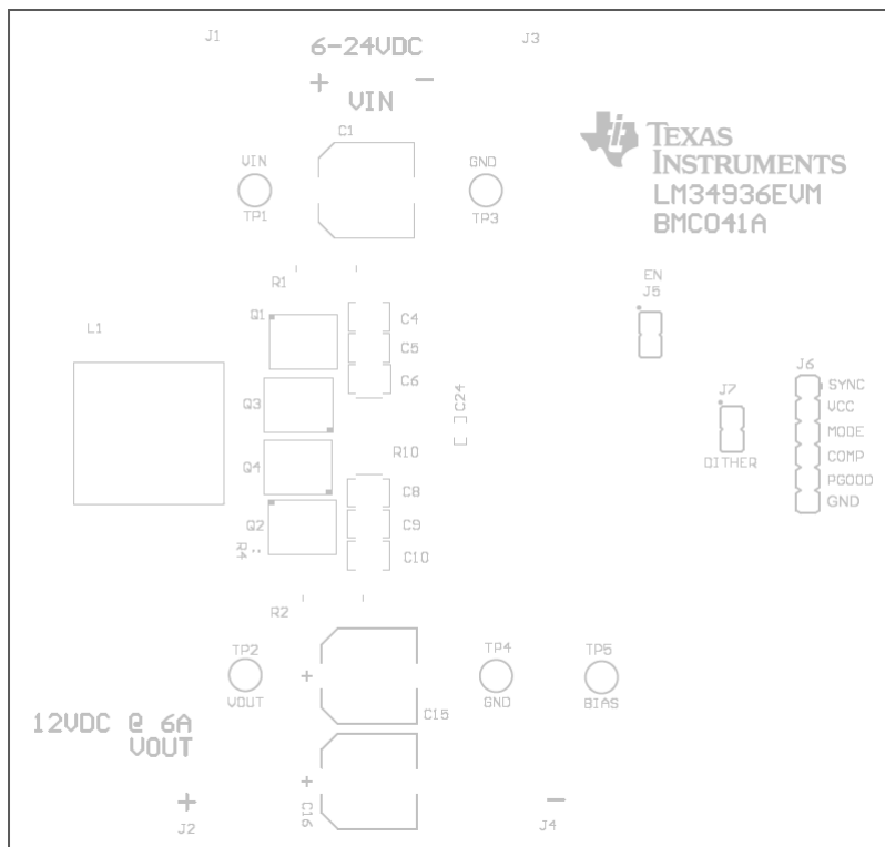
Figure 13. Top Overlay
