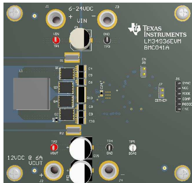
Figure 1. LM34936Evaluation Board
