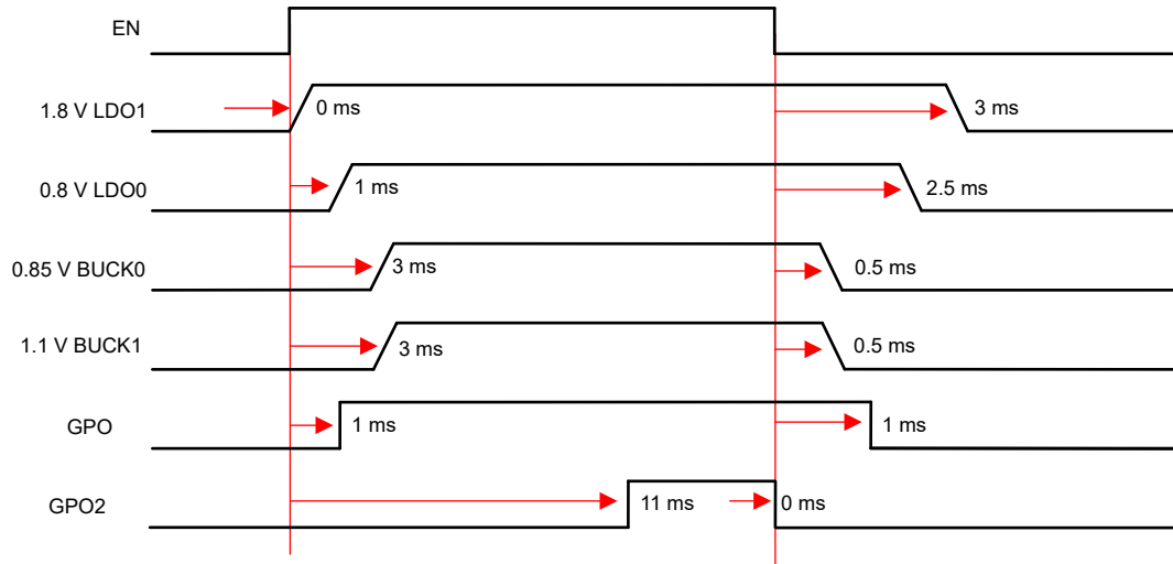
Figure 3-1. LP87334E Power-up and Power Down Sequence
