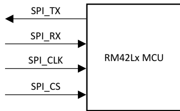
Figure 1. SPI Connections for SPI-Slave Bootloader
