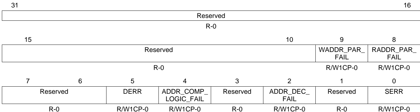
Figure 5-7. TCRAM Module Error Status Register (RAMERRSTATUS) (offset = 10h)
