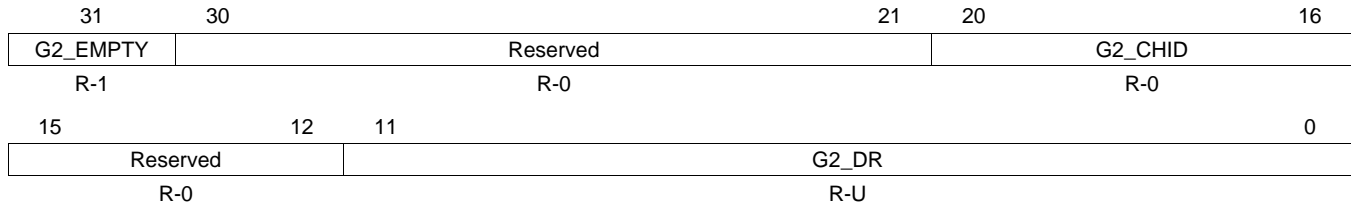
Figure 16-59. 12-bit ADC Group2 Results FIFO Register (ADG2BUFFER) [offset = D0h-EFh]
