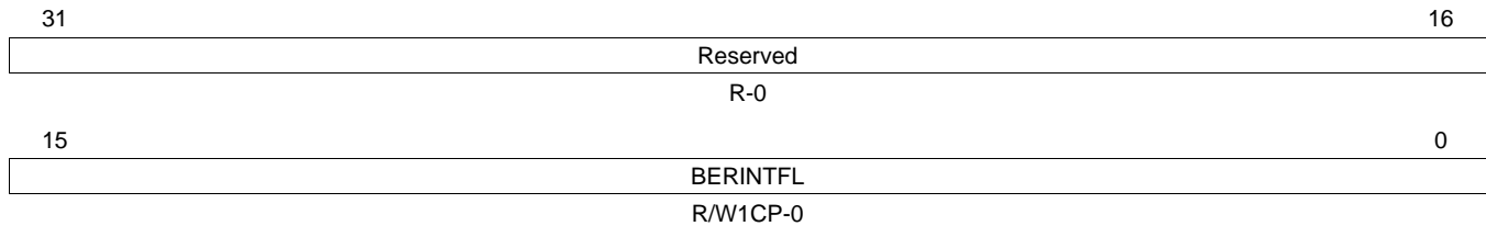
Figure 18-30. BER Interrupt Flag Register (HTU BERINTFL) [offset = 48h]
