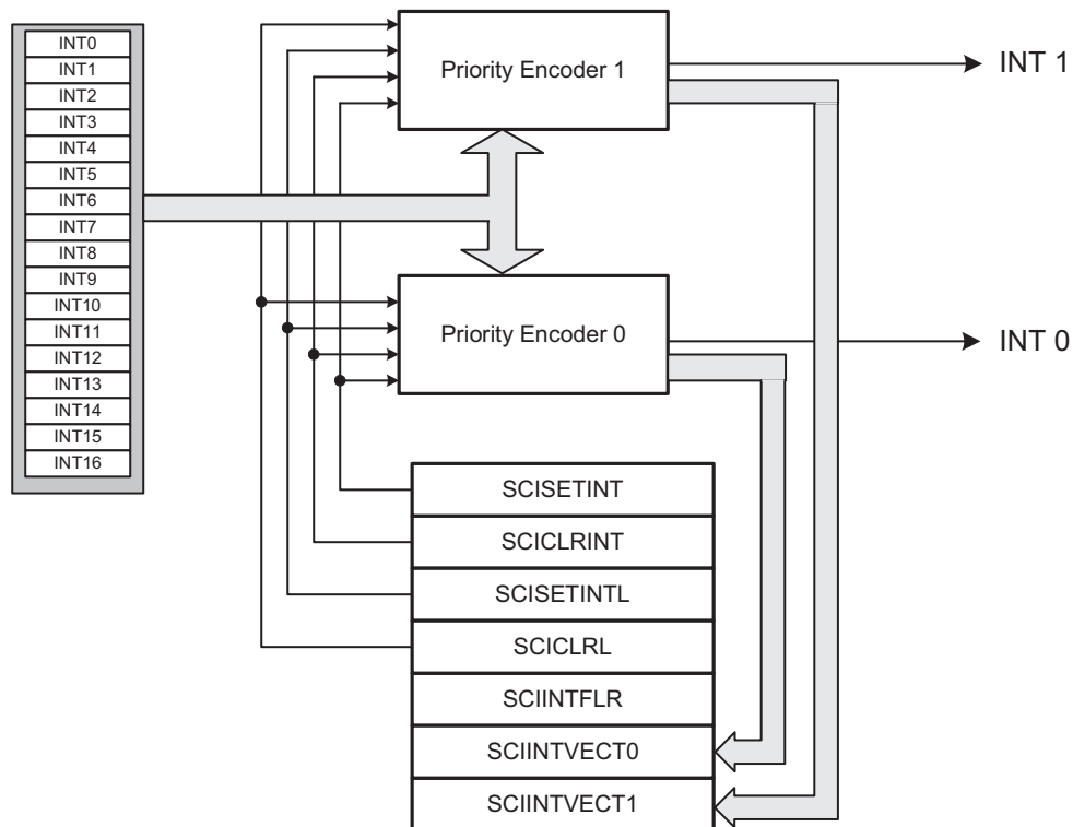
Figure 22-10. General Interrupt Scheme
