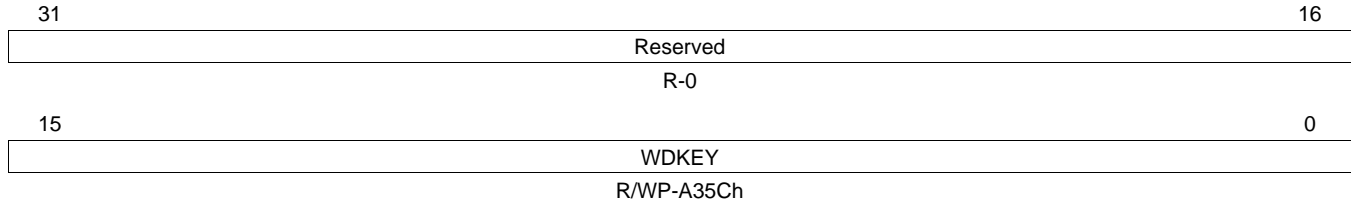
Figure 12-35. RTI Watchdog Key Register (RTIWDKEY) [offset = 9Ch]
