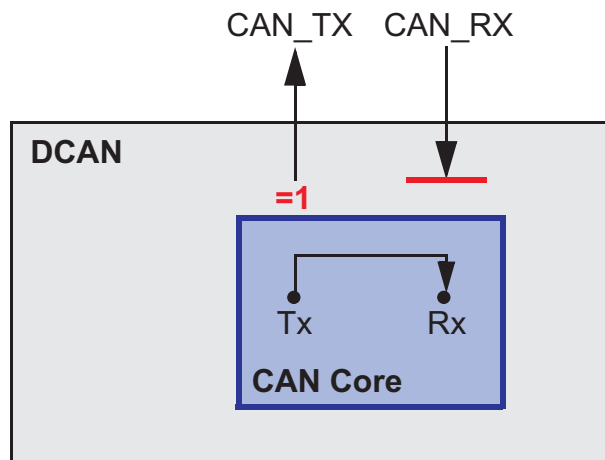
Figure 20-18. CAN Core in Loop Back Combined with Silent Mode
