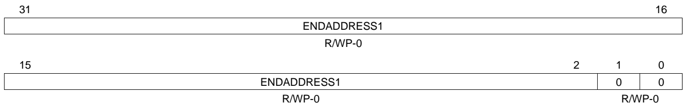
Figure 18-32. Memory Protection 1 End Address Register (HTU MP1E) [offset = 50h]
