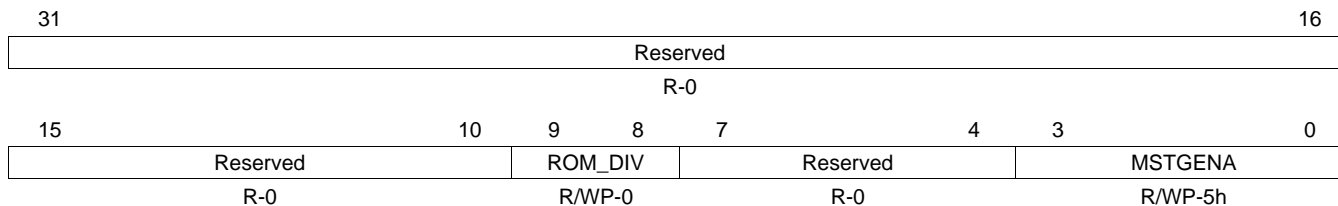
Figure 2-23. Memory Self-Test Global Control Register (MSTGCR) (offset = 58h)
