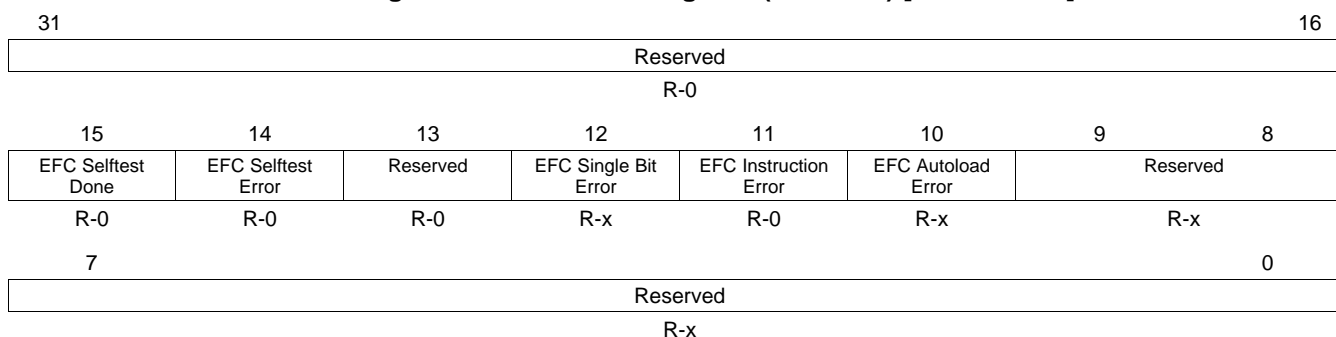
Figure 23-3. EFC Pins Register (EFCPINS) [offset = 2Ch]
