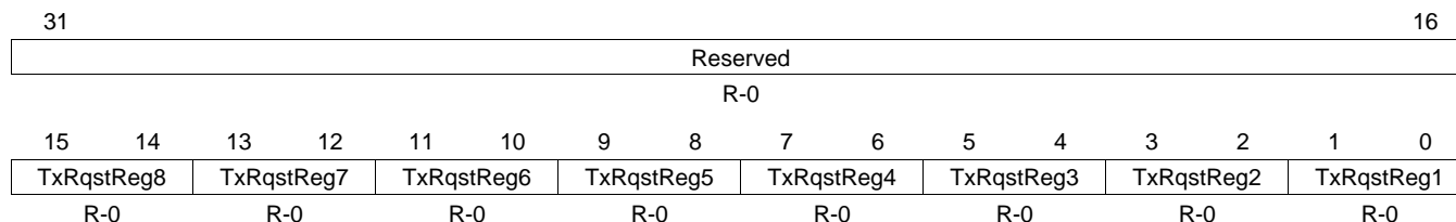
Figure 20-28. Transmission Request X Register (DCAN TXRQ X) [offset = 84h]
