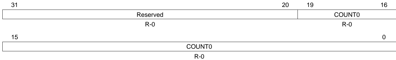
Figure 10-13. DCC Counter0 Value Register (DCCNT0) (offset = 18h)
