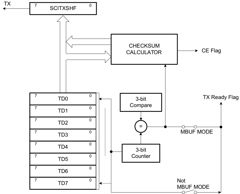
Figure 22-9. Transmit Buffers
