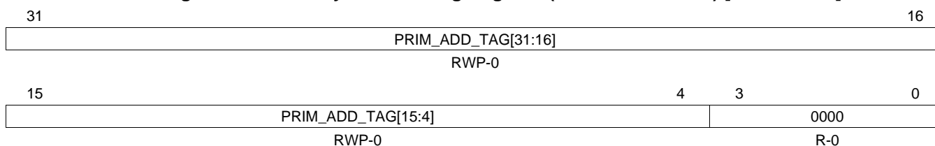
Figure 4-18. Primary Address Tag Register (FPRIM_ADD_TAG) [offset = 28h]
