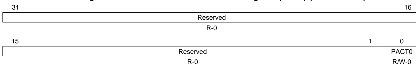
Figure 6-6. PBIST Activate/Clock Enable Register (PACT) (offset = 180h)
