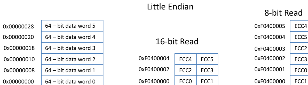
Figure 4-1. ECC Organization for Program Flash (144-Bits Wide)
