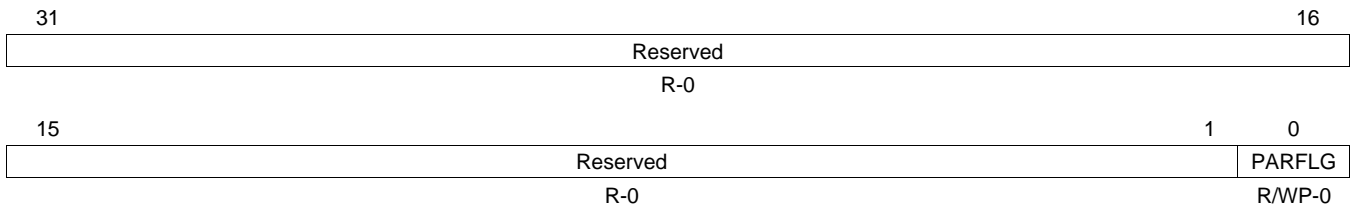
Figure 14-11. Interrupt Vector Table Parity Flag Register (PARFLG) [offset = ECh]
