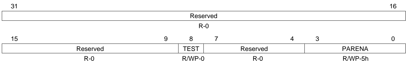
Figure 14-12. Interrupt Vector Table Parity Control Register (PARCTL) [offset = F0h]
