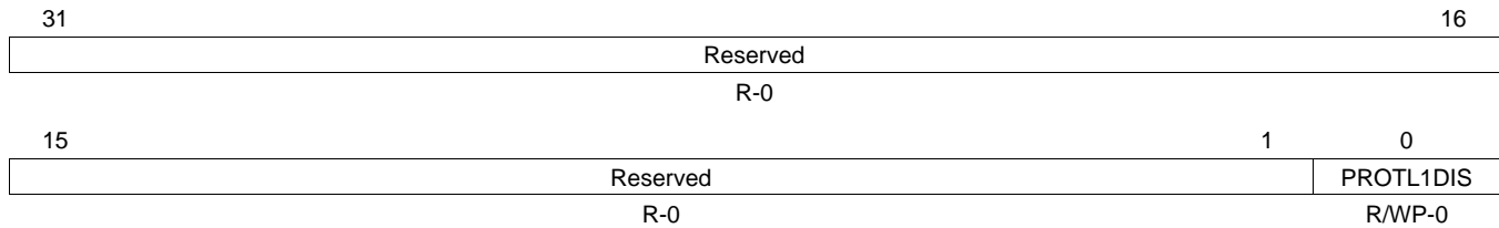
Figure 4-20. Flash Bank Protection Register (FBPROT) [offset = 30h]
