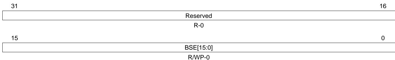
Figure 4-21. Flash Bank Sector Enable Register (FBSE) [offset = 34h]
