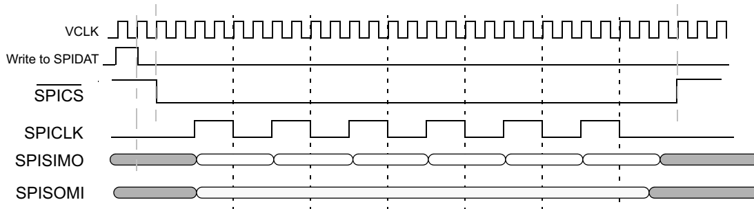
Figure 21-69. SPI/MibSPI Pins During Master Mode 4-pin with \overline{\text{SPIC}}\overline{\text{S}} Configuration
