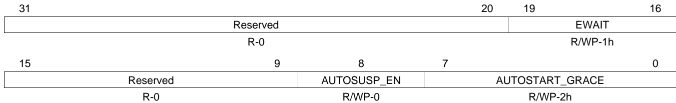
Figure 4-42. EEPROM Emulation Configuration Register (EEPROM_CONFIG) [offset = 2B8h]
