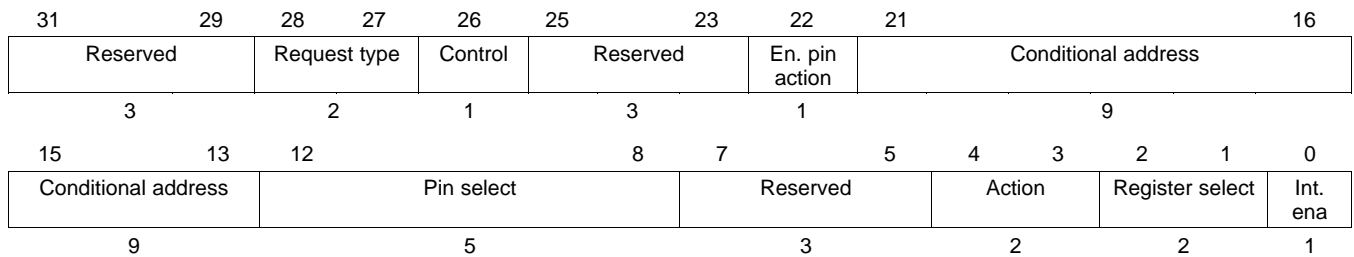
Figure 17-126. PWCNT Control Field (C31:C0)
