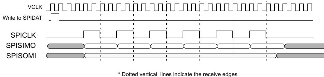
Figure 21-68. SPI/MibSPI Pins During Master Mode 3-pin Configuration
