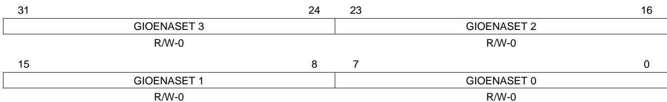
Figure 19-8. GIO Interrupt Enable Set Register (GIOENASET) [offset = 10h]
