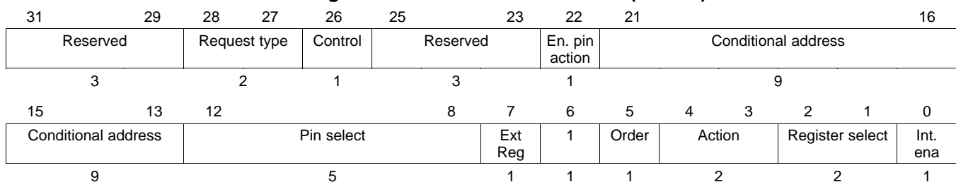
Figure 17-109. MCMP Control Field (C31:C0)
