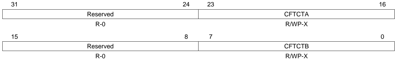
Figure 18-48. Current Frame Count Register (HTU CFCOUNT) [offset = 108h]
