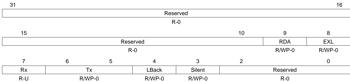
Figure 20-24. Test Register (DCAN TEST) [offset = 14h]
