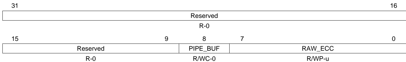
Figure 4-37. Uncorrected Raw ECC Register (FRAW_ECC) [offset = 78h]
