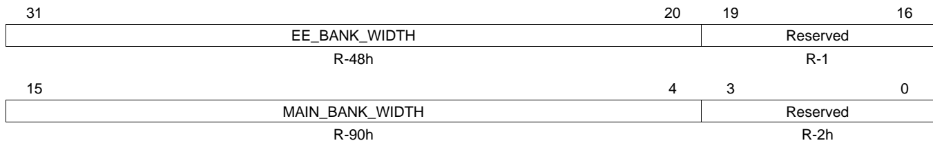
Figure 4-50. Flash Bank Configuration Register (FCFG_BANK) [offset = 400h]
