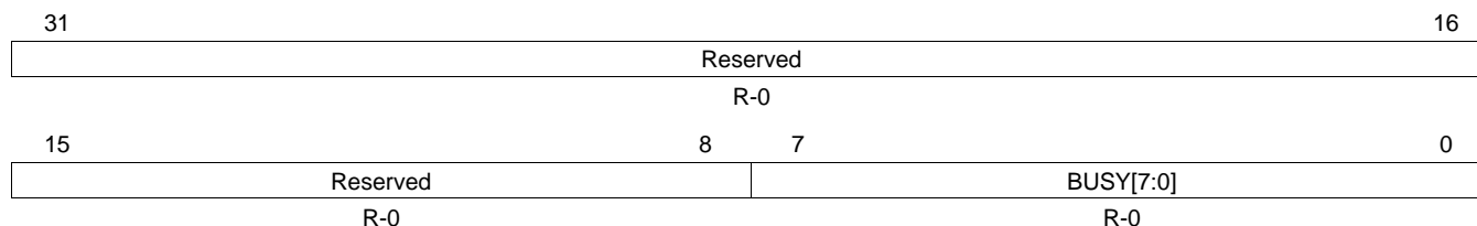
Figure 4-22. Flash Bank Busy Register (FBBUSY) [offset = 38h]
