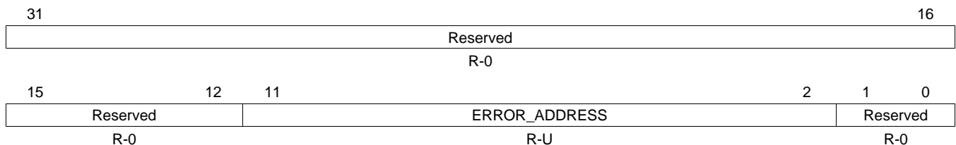
Figure 16-93. ADC Parity Error Address Register (ADPARADDR) [offset = 184h]
