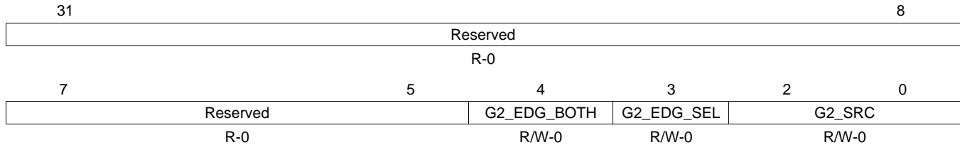
Figure 16-30. ADC Group2 Trigger Source Select Register (ADG2SRC) [offset = 24h]
