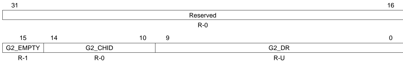
Figure 16-60. 10-bit ADC Group2 Results' FIFO Register (ADG2BUFFER) [offset = D0h-EFh]
