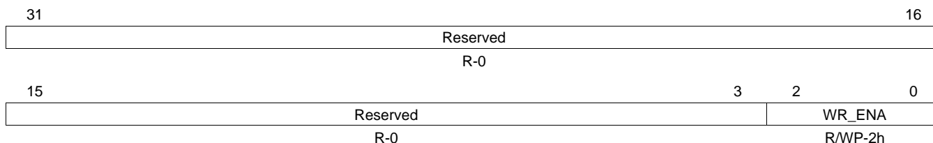
Figure 4-40. FSM Register Write Enable (FSM_WR_ENA) [offset = 288h]
