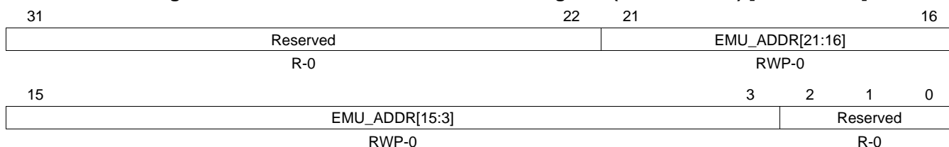
Figure 4-33. EEPROM Emulation Address Register (FEMU_ADDR) [offset = 68h]
