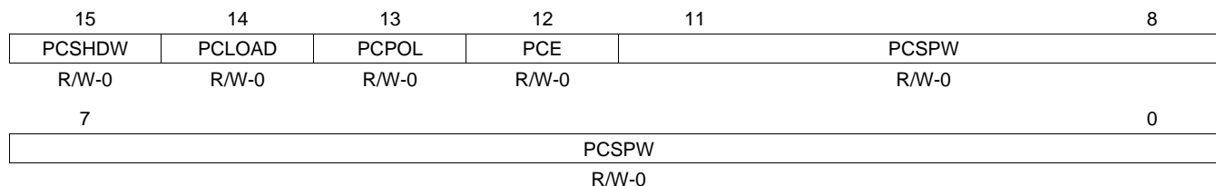
Figure 15-35. eQEP Position-compare Control (QPOSCTL) Register (offset = 2Eh)
