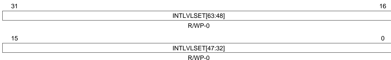
Figure 11-31. ESM Interrupt Level Set Register 4 (ESMILSR4) [address = FFFF F550h]
