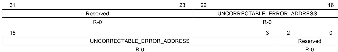
Figure 5-9. TCRAM Module Uncorrectable Error Address Register (RAMUERRADDR) (offset = 1Ch)
