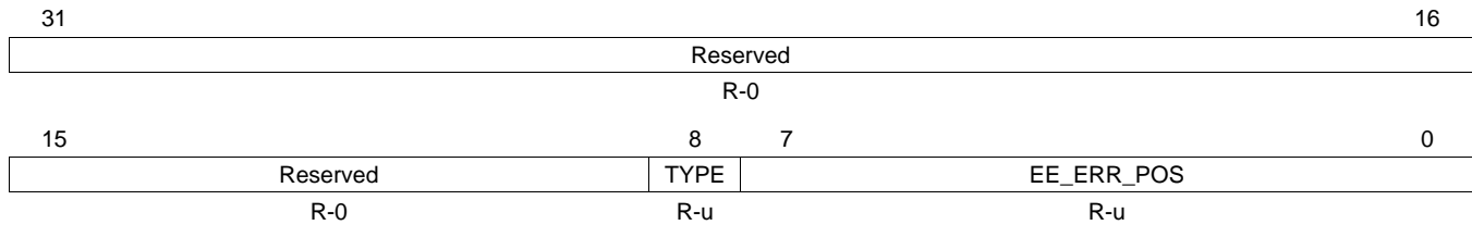
Figure 4-47. EEPROM Emulation Correctable Error Position Register (EE_COR_ERR_POS) [offset = 318h]
