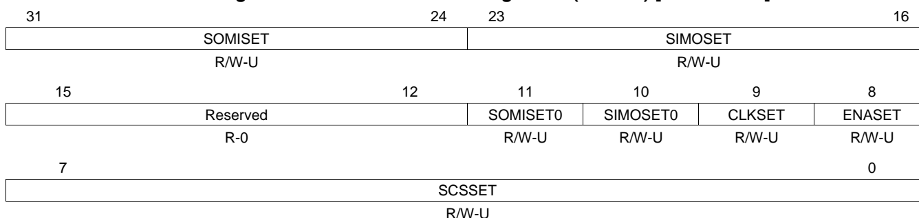
Figure 21-26. SPI Pin Control Register 4 (SPIPC4) [offset = 24h]
