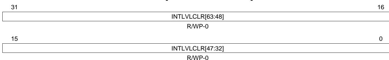
Figure 11-32. ESM Interrupt Level Clear Register 4 (ESMILCR4) [address = FFFF F554h]
