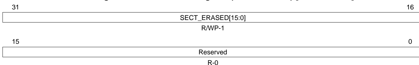
Figure 4-41. FSM Sector Register (FSM_SECTOR) [offset = 2A4h]
