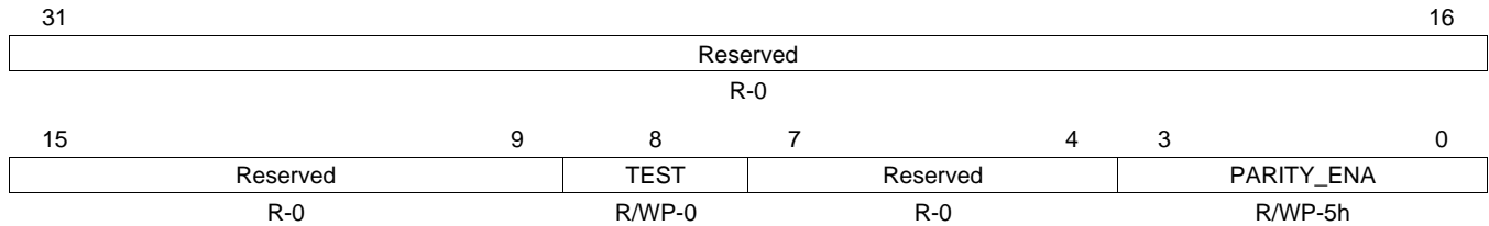
Figure 16-92. ADC Parity Control Register (ADPARCR) [offset = 180h]
