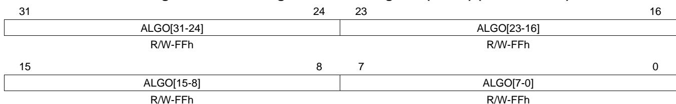
Figure 6-17. ROM Algorithm Mask Register (ALGO) (offset = 1C4h)
