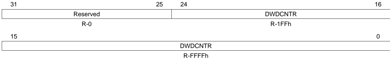
Figure 12-36. RTI Watchdog Down Counter Register (RTIDWDCNTR) [offset = A0h]
