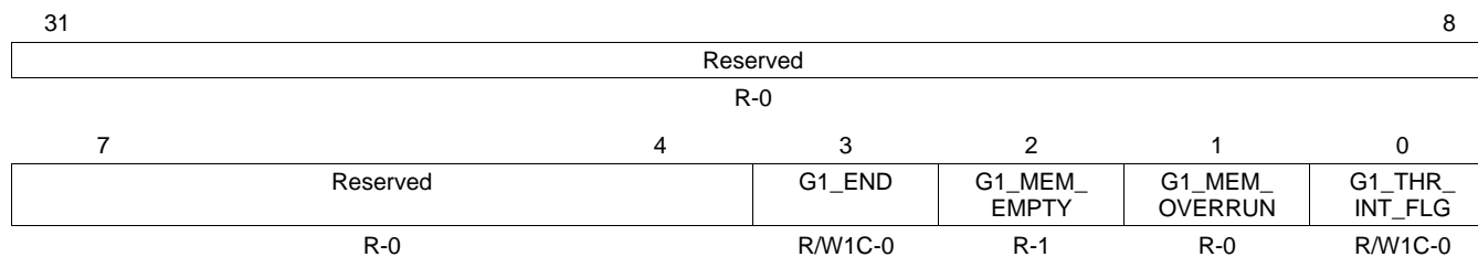
Figure 16-35. ADC Group1 Interrupt Flag Register (ADG1INTFLG) [offset = 38h]
