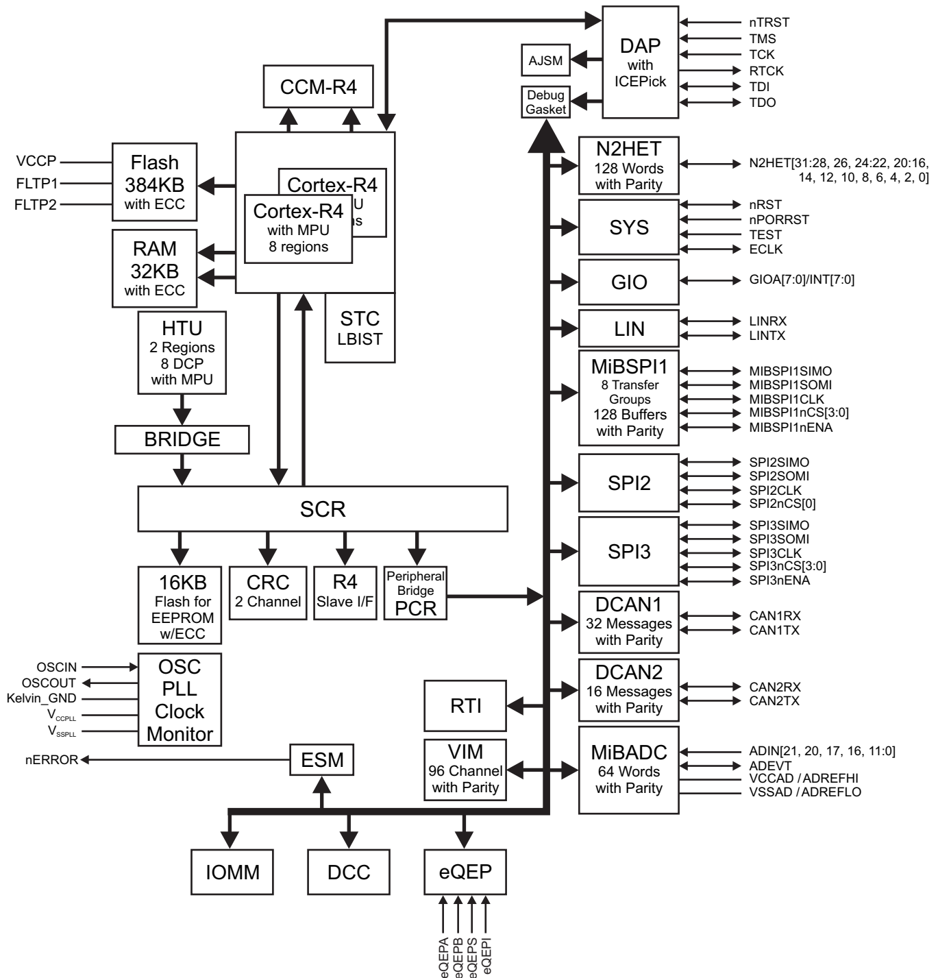
Figure 1-1. Block Diagram
