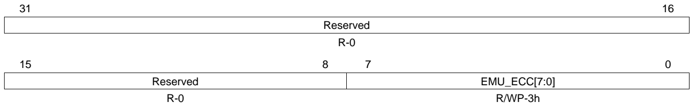
Figure 4-32. EEPROM Emulation ECC Register (FEMU_ECC) [offset = 60h]
