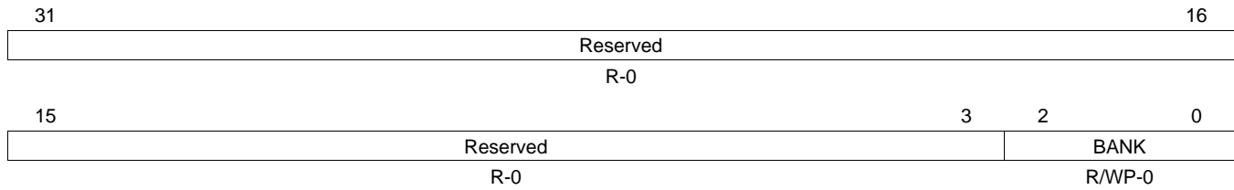
Figure 4-28. Flash Module Access Control Register (FMAC) [offset = 50h]
