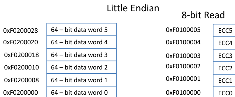
Figure 4-2. ECC Organization for Bank 7 (72-Bits Wide)
