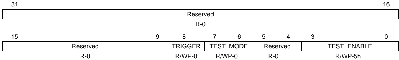
Figure 5-10. TCRAM Module Test Mode Control Register (RAMTEST) (offset = 30h)
