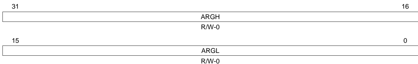
Figure 23-31. MMC Argument Register (MMCARGHL)
