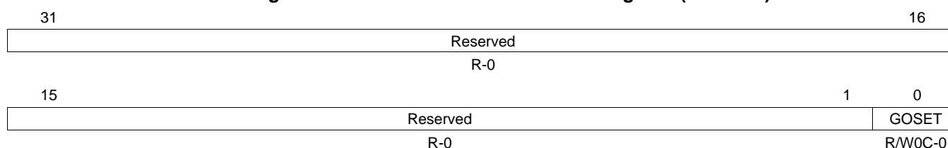
Figure 7-15. PLL Controller Command Register (PLLCMD)
