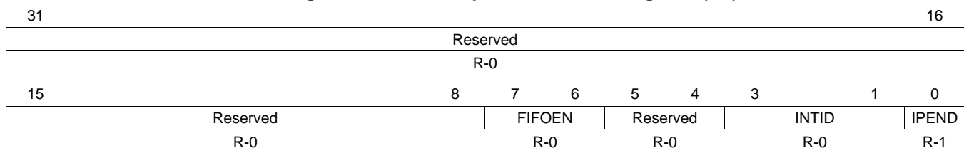
Figure 26-12. Interrupt Identification Register (IIR)
