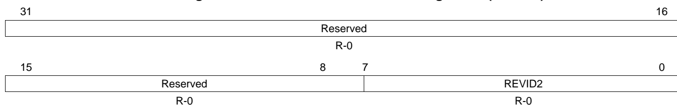
Figure 26-22. Revision Identification Register 2 (REVID2)
