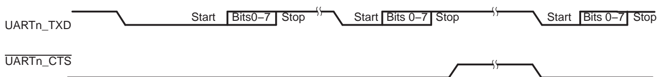
Figure 26-7. Autoflow Functional Timing Waveforms for \overline{\text{UARTn\_CTS}}
