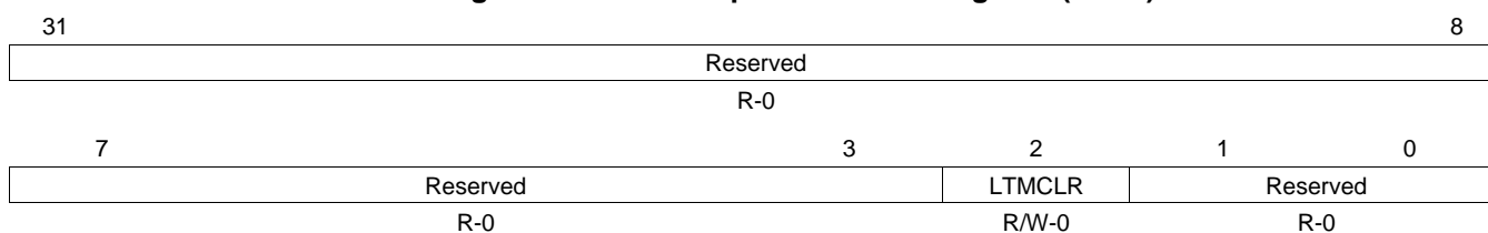
Figure 19-28. Interrupt Mask Clear Register (IMCR)
