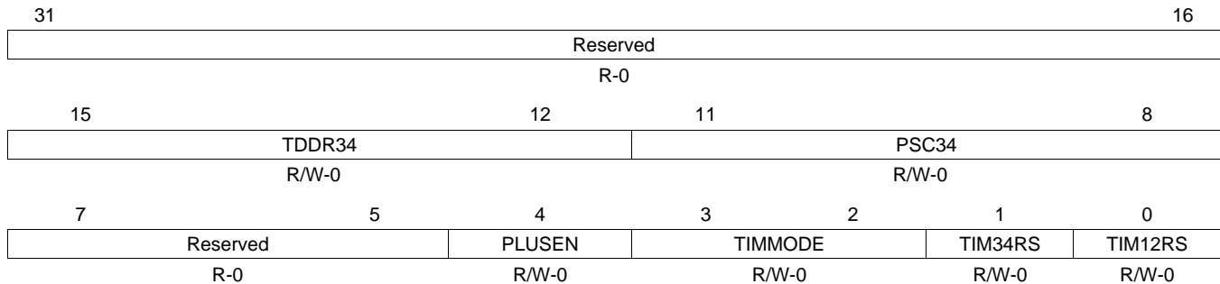
Figure 25-22. Timer Global Control Register (TGCR)
