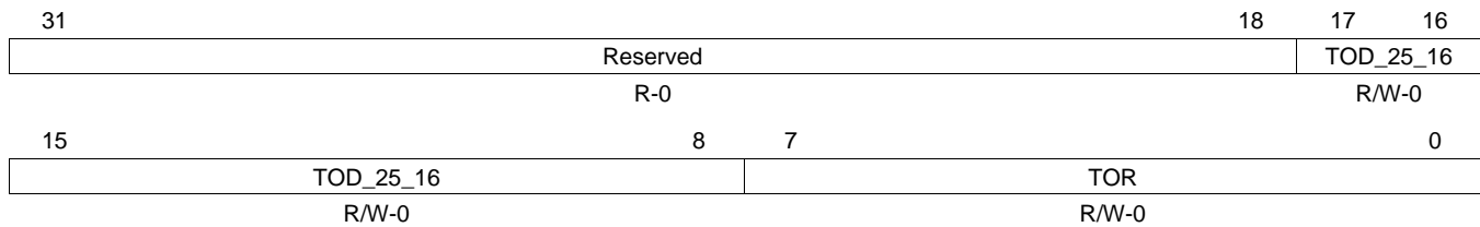
Figure 23-22. MMC Response Time-Out Register (MMCTOR)
