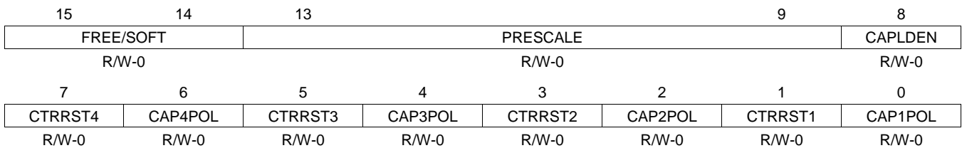
Figure 13-23. ECAP Control Register 1 (ECCTL1)
