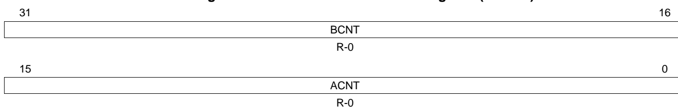
Figure 16-93. Source Active Count Register (SACNT)
