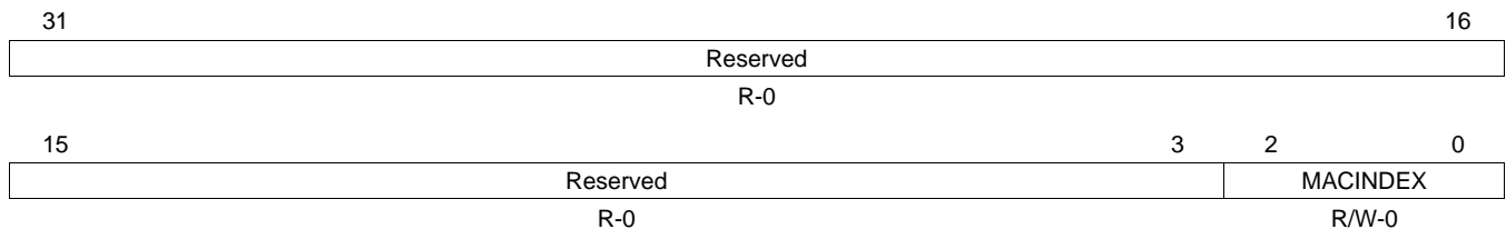
Figure 17-83. MAC Index Register (MACINDEX)
