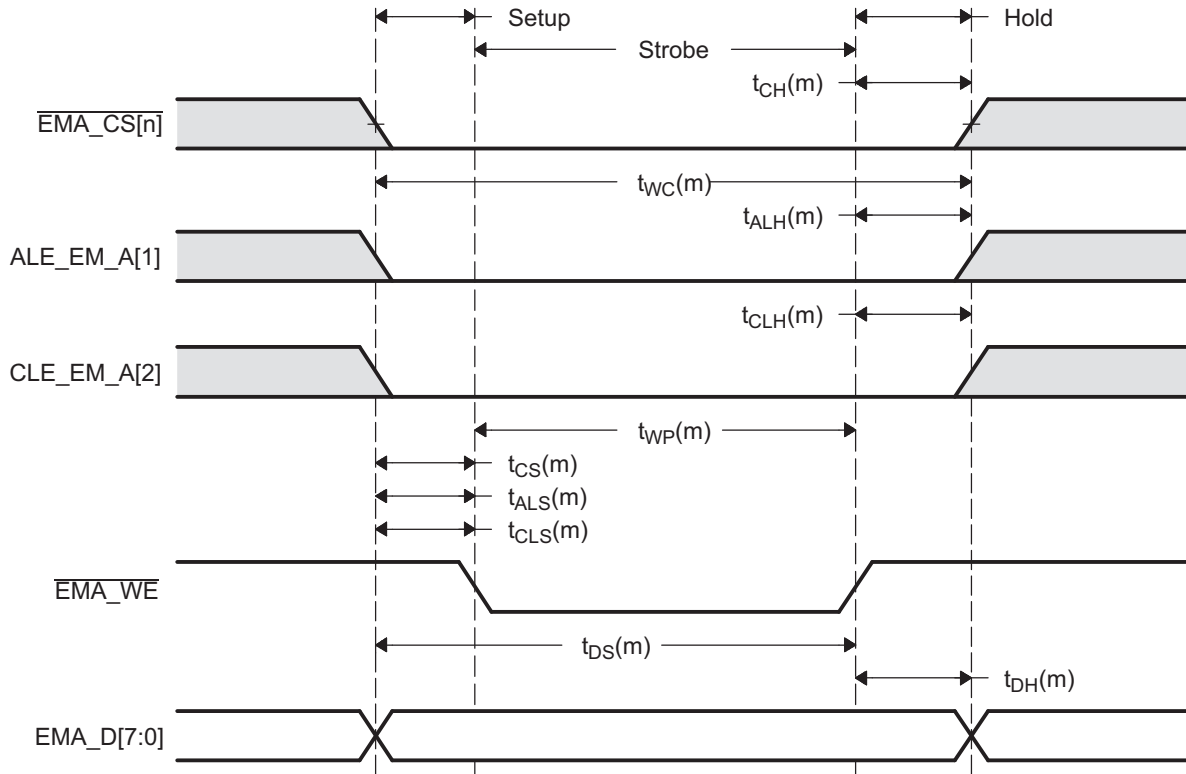
Figure 18-30. Timing Waveform of a NAND Flash Data Write
