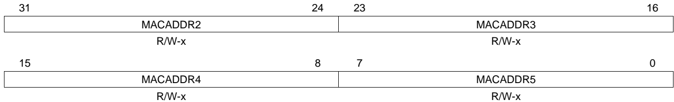
Figure 17-82. MAC Address High Bytes Register (MACADDRHI)
