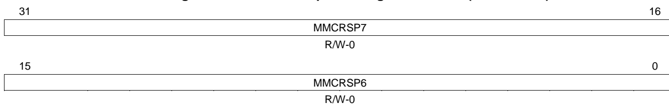
Figure 23-35. MMC Response Register 6 and 7 (MMCRSP67)
