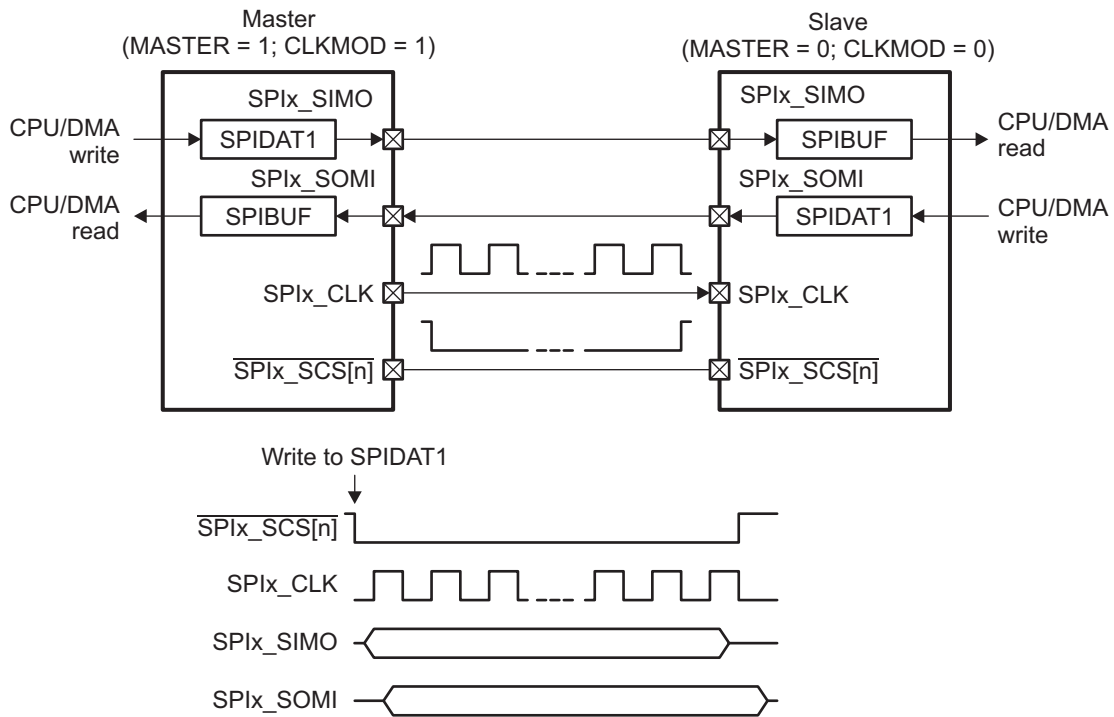
Figure 24-3. SPI 4-Pin Option with SPIx_SCS[n]
