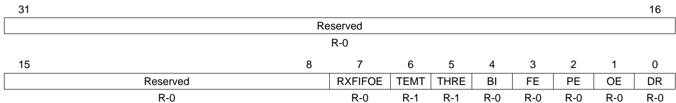
Figure 26-16. Line Status Register (LSR)
