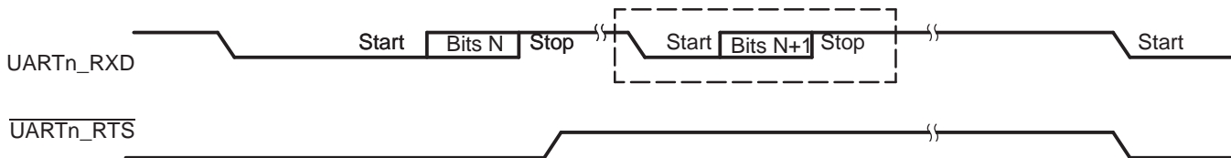
Figure 26-6. Autoflow Functional Timing Waveforms for \overline{\text{UARTn\_RTS}}
