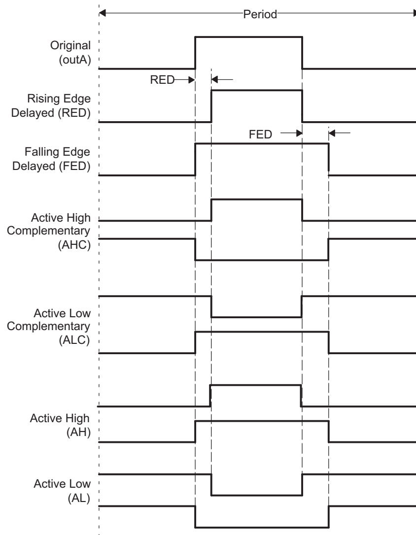
Figure 14-30. Dead-Band Waveforms for Typical Cases ( 0\% < \text{Duty} < 100\% )
