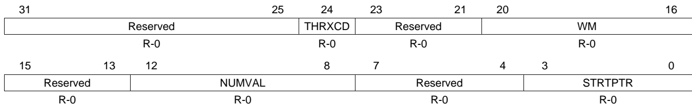
Figure 16-58. Queue n Status Register (QSTAT n )
