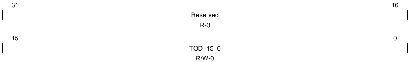
Figure 23-23. MMC Data Read Time-Out Register (MMCTOD)
