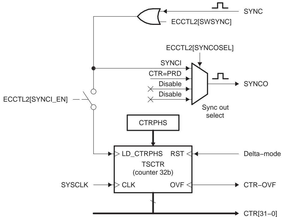
Figure 13-7. Counter and Synchronization Block Diagram
