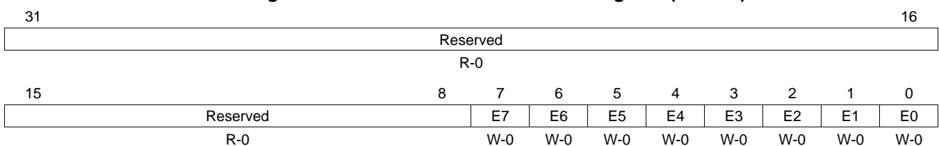
Figure 16-79. QDMA Event Enable Set Register (QEESR)
