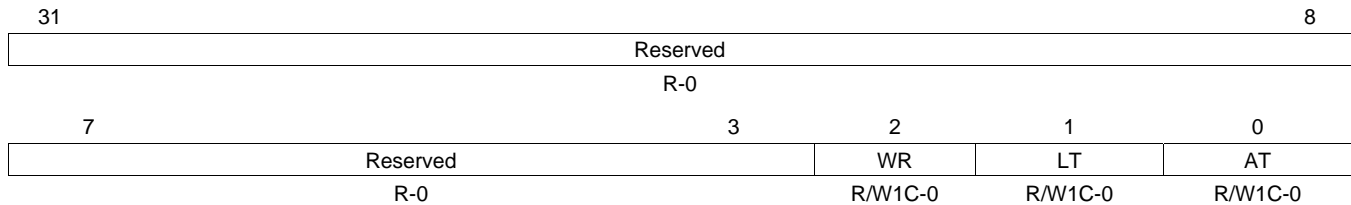
Figure 18-38. EMIFA Interrupt Raw Register (INTRAW)
