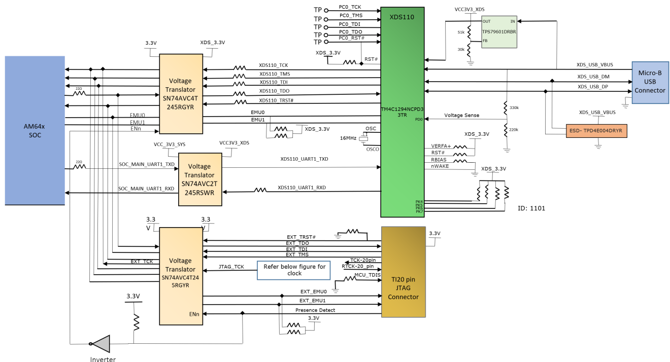
Figure 2-11. JTAG Interface
