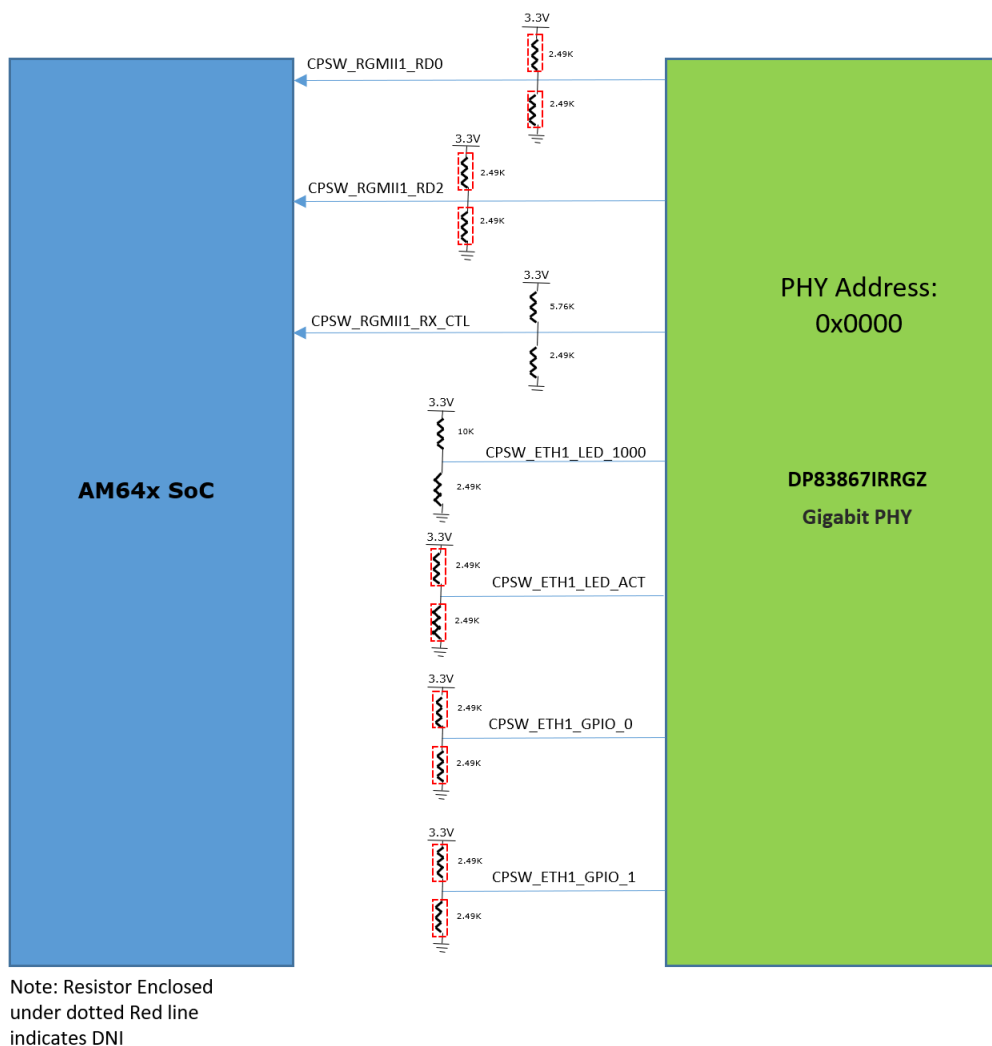
Figure 2-19. CPSW Ethernet PHY-1 Strap Settings
