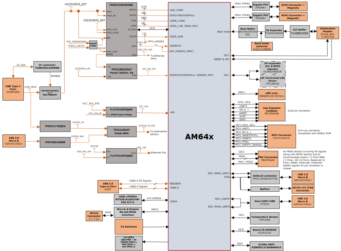
Figure 2-3. Starter Kit Processor Board Functional Block Diagram
