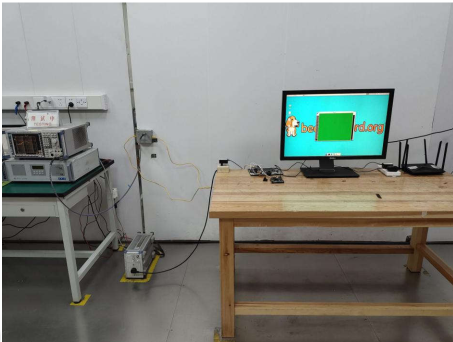
CONDUCTED DISTURBANCE TEST SETUP-2
