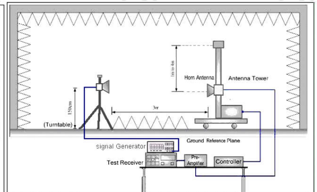
Figure 2. Above 1GHz
