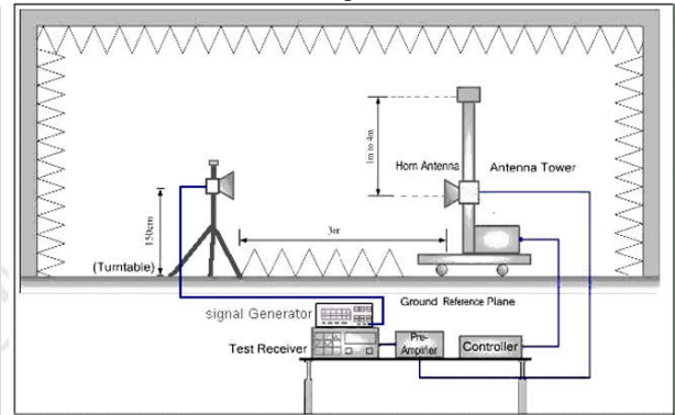
Figure 2. Above 1GHz
