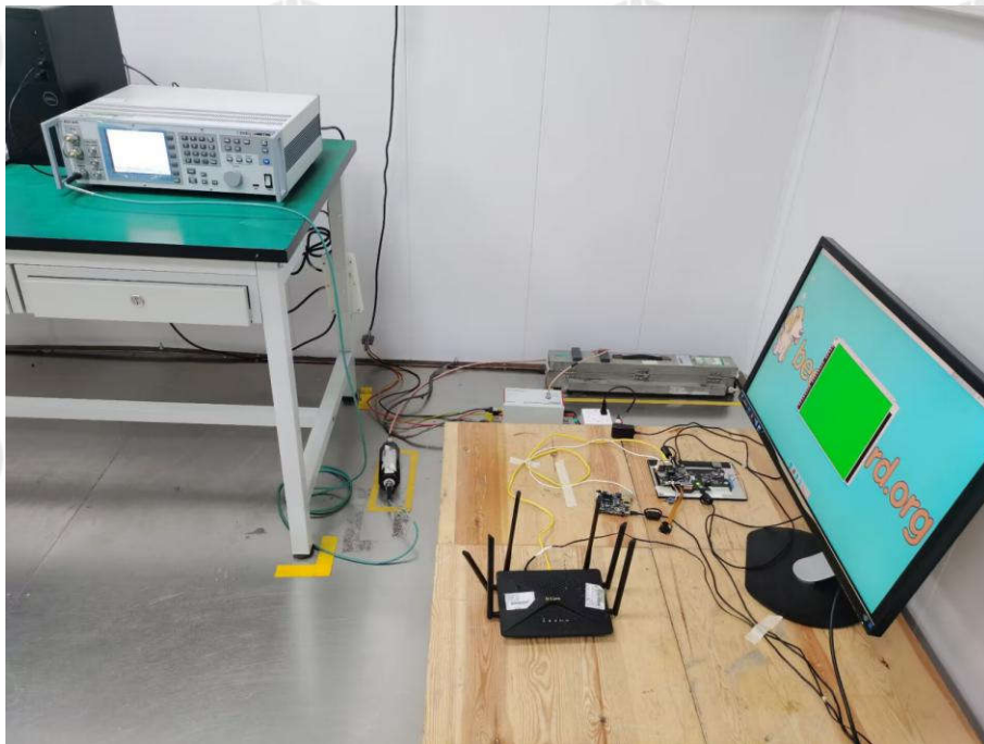
RADIO-FREQUENCY CONTINUOUS CONDUCTED IMMUNITY TEST SETUP
