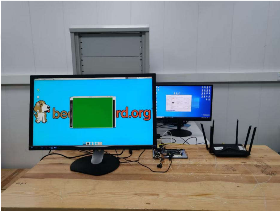
VOLTAGE DIPS AND INTERRUPTIONS TEST SETUP
