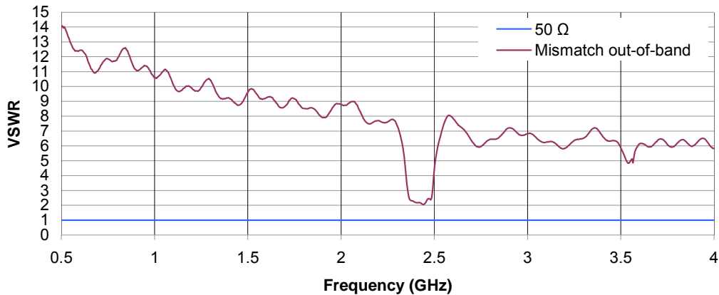
Figure 6.2 VSWR
