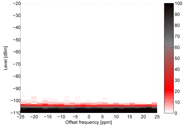
Figure 8. C-Mode 100 kbps, \pm 33.75 kHz, 10-Byte Payload
