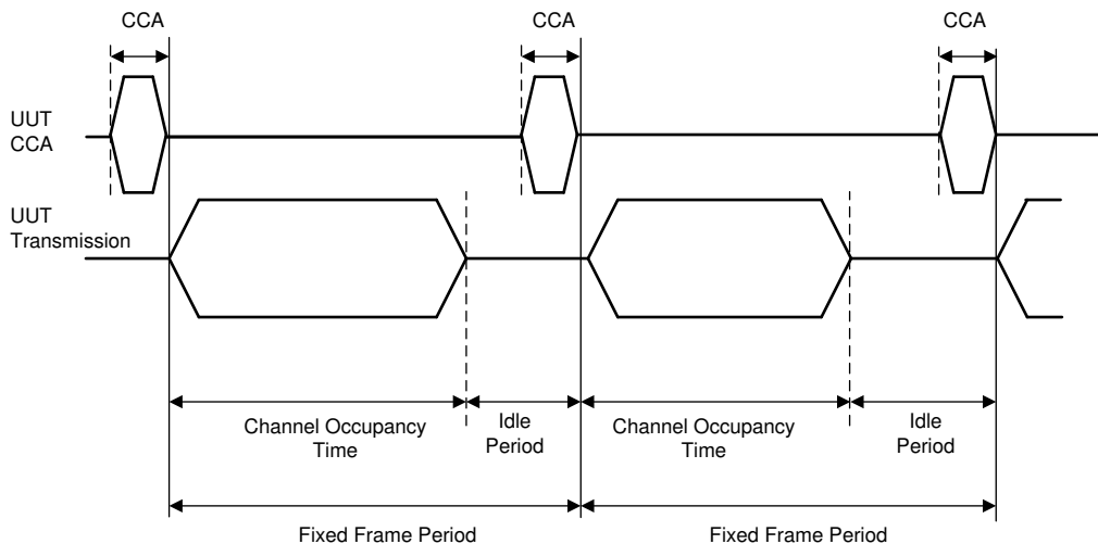
Figure 6-2. Example of timing for Frame Based Equipment
