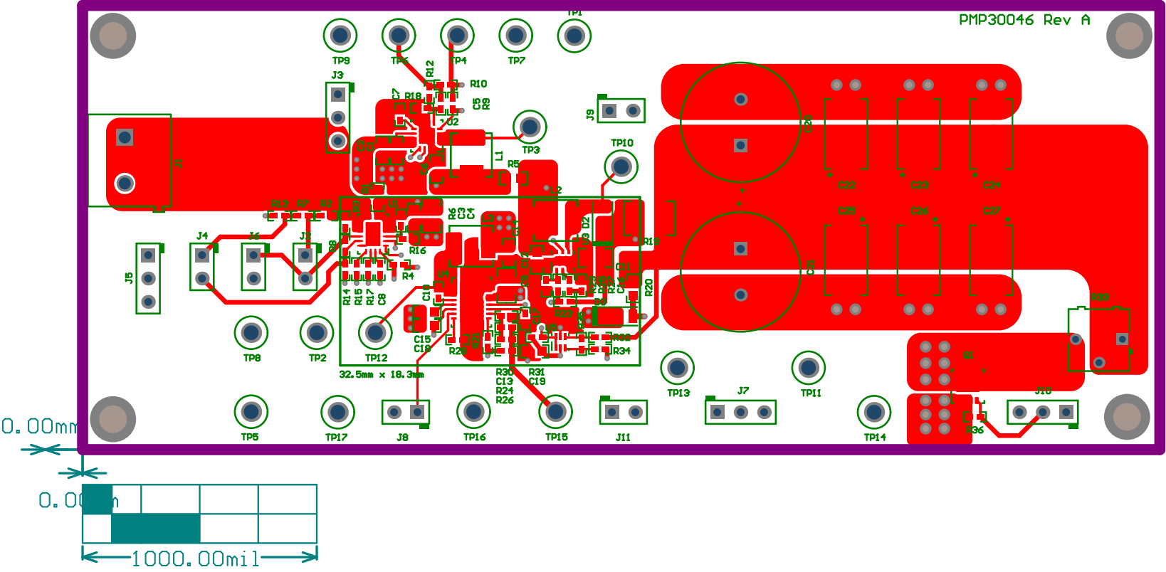
PCB Board Dimensions
