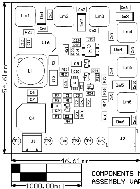
M1 Board Outline
